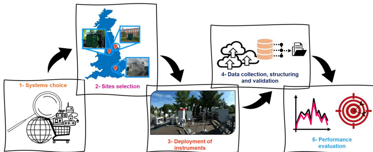
Fig. 1 Main QUANT study workflow description: first, market research was conducted to identify and select suitable sensor systems; second, three urban sites in the UK were chosen for implementation; third, commercial devices were installed in the selected locations; fourth, the collection, organization and preliminary validation of the data was carried out; fifth, performance assessment (not part of this paper). For the WPS, steps 1 and 2 differed slightly, as participation was voluntary (no selection on our part) and took place at a single site (MAQS). See the methods section for more details.
