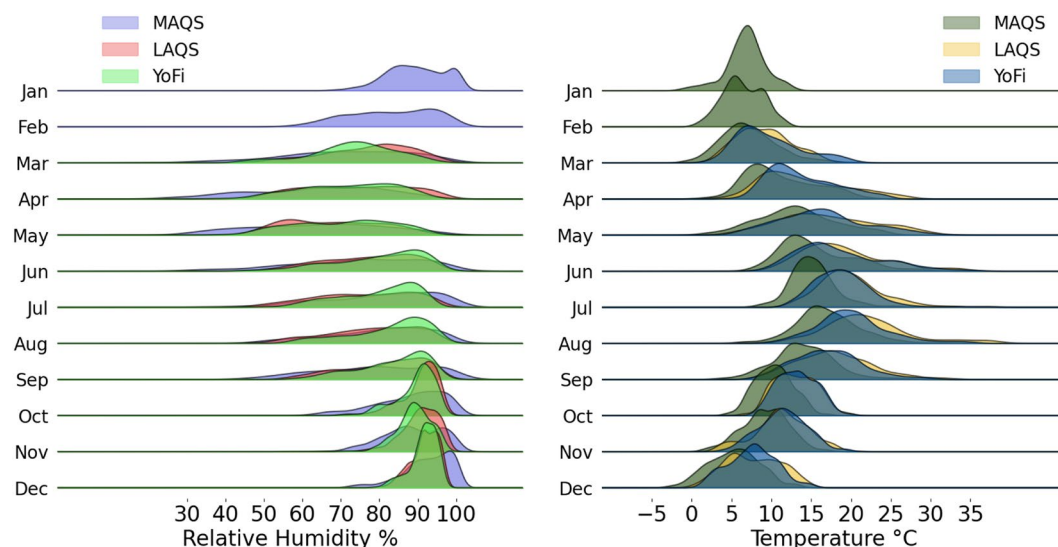
Fig. 3 Hourly distribution of Relative Humidity (%) (left panel) and Temperature (°C; right panel) for 2020 across three locations: MAQS (year-round), LAQS, and YoFi (the latter two from March onwards). These plots capture the seasonal variation of these key environmental parameters influencing sensor data quality.
