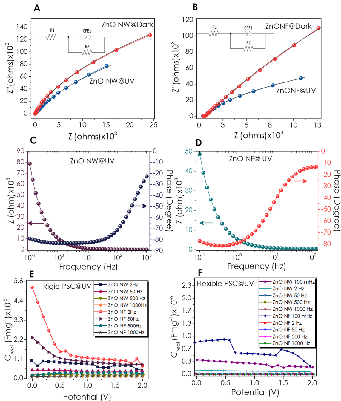
Figure 8. EIS measurements were performed in the scan range: 1 MHz to 0.1 Hz at 0 V. Nyquist Plot; (A) ZnO NW, (B) ZnO NF (The symbols stand for experimental data; the solid lines are the curves fitted to the electrical circuit model depicted in the inset), Bode plots (C) ZnO NW and (D) ZnO NF, Areal Capacitance at various frequencies at UV light (E) ZnO NW, (F) ZnO NF.
