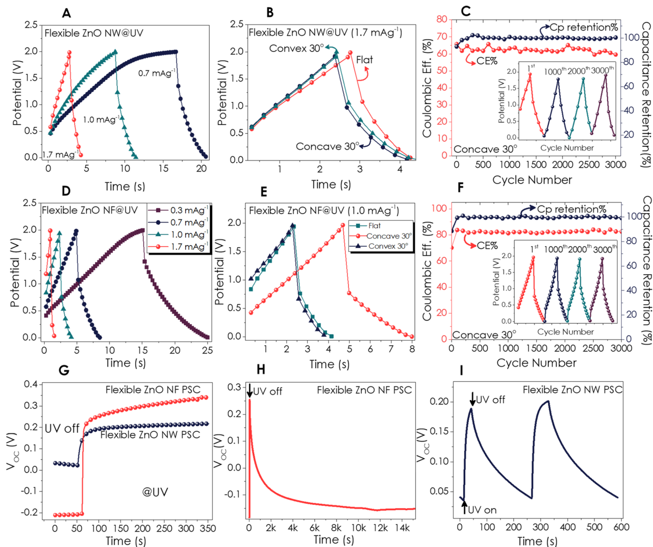
Figure 7. GCD curves for Flexible ZnO NW P-SCs; (A) at various current densities under UV light, (B) comparison of the GCD curves of flat and bent P-SC, (C) CE% and capacitance retention of concave P-SC, GCD curves for Flexible ZnO NF; (D) at various current densities under UV light, (E) comparison GCD curves of flat and bent P-SC, (F) CE% and capacitance retention of concave P-SC; Open circuit potential ( V_{OC} ) curves; (G) at dark and under UV illumination for 5 min, V_{OC} response to chopped light and relaxation duration for flexible (H) ZnO NF and (I) NW P-SC devices.
