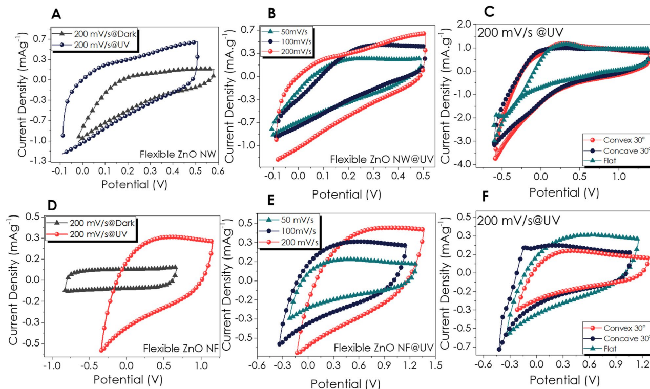
Figure 6. CV curves of flexible ZnO NW based P-SC; (A) with 200 mV s -1 scan rate under UV and dark conditions, (B) under UV light with different scan rates, (C) bent and flat P-SC with 200 mV s -1 scan rate; and flexible ZnO NF based P-SC; (D) with 200 mV s -1 scan rate under UV and dark conditions, (E) under UV light with different scan rates, (F) bent and flat P-SC with 200 mV s -1 scan rate.
