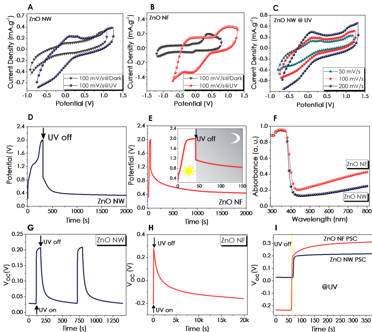
Figure 4. CV curves of (A) ZnO NW and (B) ZnO NF at dark and UV conditions, (C) ZnO NW at UV with various scan rates. The curves for photo-charging (at 0.55 \text{ mA g}^{-1} )/self-discharge in the dark under zero applied current after long-term P-SC devices; (D) ZnO NW, (E) ZnO NF, (F) UV-Vis Absorbance curves for both thin-film P-SC devices; Changes in open circuit potential ( V_{oc} ) under UV illumination and dark conditions for (G) ZnO NW, (H) ZnO NF and (I) Comparison for V_{oc} at dark and under UV illumination for 5 min.
