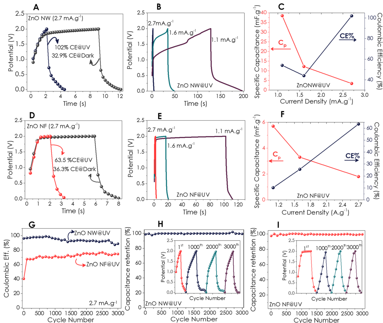
Figure 5. GCD curves; (A) comparison for ZnO NW under UV light and dark conditions at a 2.7 \text{ mA g}^{-1} current density, (B) depending on changing current density under UV illumination, (C) capacitance and Coulombic efficiency, (D) comparison for ZnO NF under UV light and dark condition at 2.7 \text{ mA g}^{-1} current density, (E) depending on changing current density under UV illumination, (F) capacitance and Coulombic efficiency, (G) Coulombic efficiency retention for 3000 cycles GCD under UV illumination. Capacitance retention and 1st, 1000th, 2000th and 3000th charge–discharge cycles (inset figure) for (H) ZnO NW and (I) ZnO NF.
