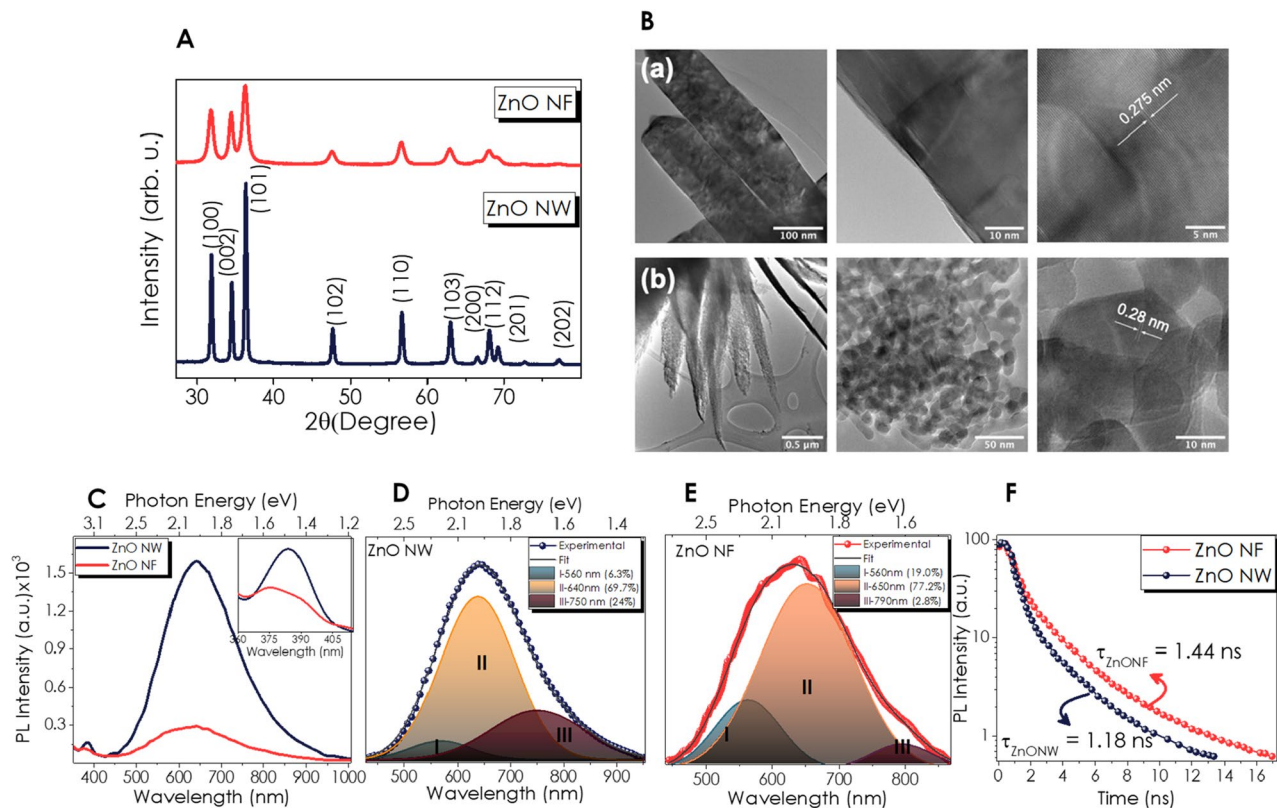
Figure 1. (A) XRD patterns; (B) TEM and HRTEM (a) NW and (b) NF; normalized PL spectra (C) Comparison of NF and NW, deconvoluted DLE of (D) NW, (E) NF powder; (F) Tr-PL curves.
