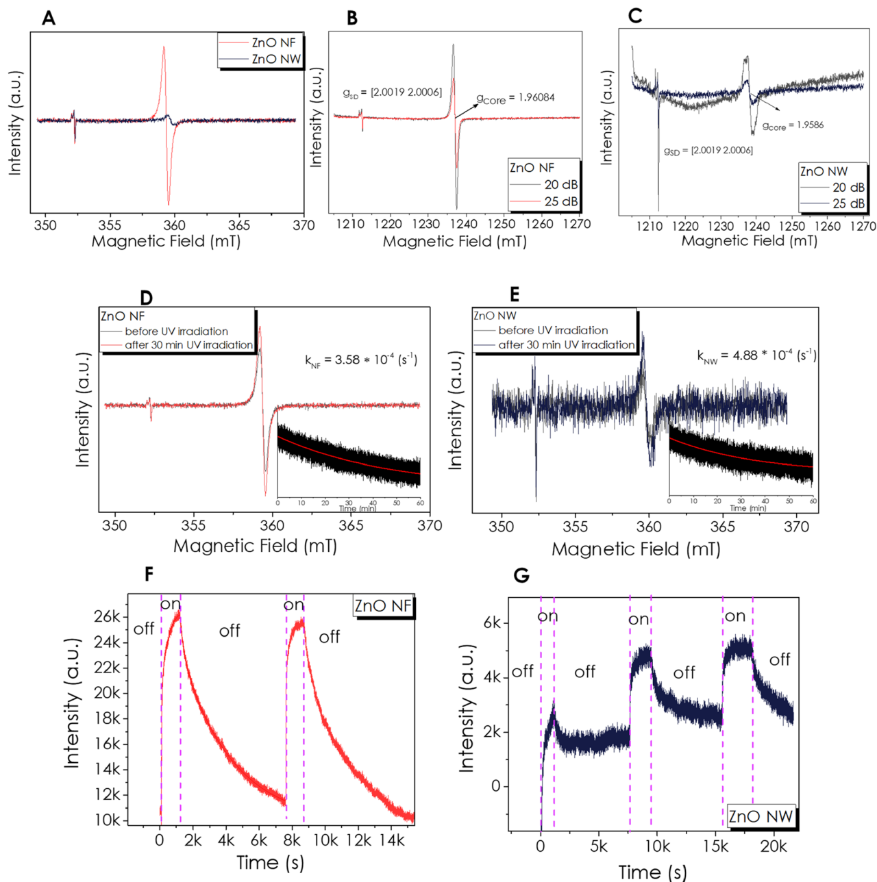
Figure 2. (A) X-band EPR spectra (9.879 GHz) of the ZnO-based materials, Q-band EPR spectra (33.984 GHz) of the NF (B), and NW (C), EPR spectra of the two in dark conditions (black line) and subsequent the irradiation time (red line) of (D) NF and (E) NW. The insets show the evolution of the EPR signal maximum after the UV-light excitation was stopped, EPR signal evolution during on-off UV-light cycles of (F) NF and (G) NW samples.
