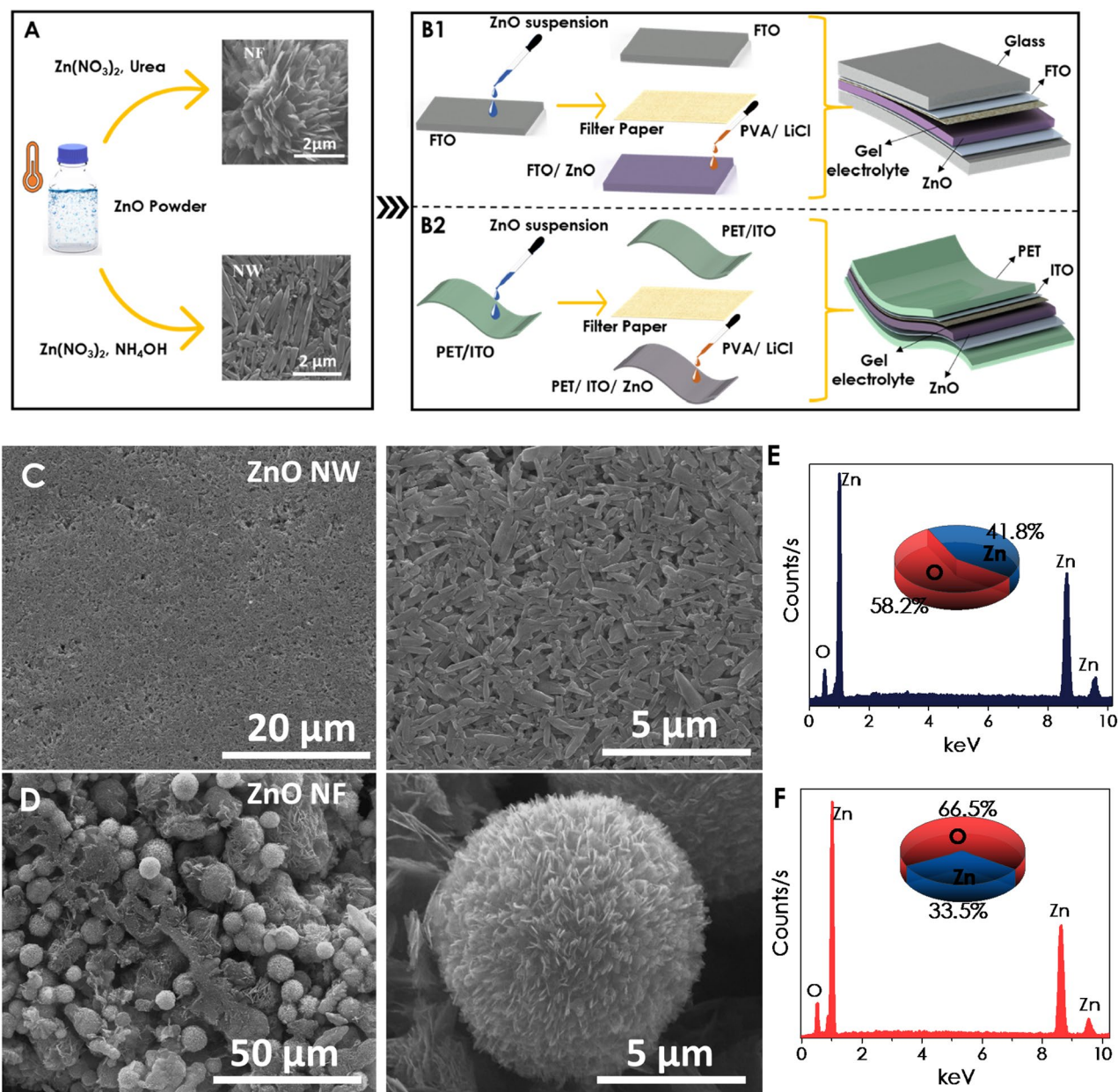
Figure 3. (A) Schematic demonstration for ZnO powder preparation, (B) the rigid and flexible P-SC assemble, respectively; ESEM images of ZnO (C) NW and (D) NF powder after spin-coated on FTO coated glass substrates; and EDX analysis results of ZnO (E) NW and (F) NF.
