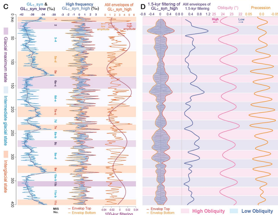
Figure 5. Comparison of millennial-scale variation patterns between the Cretaceous lacustrine deposits ( A,B ) and the late Pleistocene Greenland temperature record ( C,D ). ( A ) Lithology, log (Ca/Ti) with 5-kyr smoothing, high frequency (<5-kyr) variations of log (Ca/Ti) with envelope top and bottom (2.5-kyr sliding windows), and AM envelopes (subtraction of envelope top and bottom) of log (Ca/Ti) high frequency with its AM of 100-kyr filter (purple; frequency: 9.5e-6; bandwidth: 5.0e-6) for a ~355-kyr interval of CSH01 core. ( B ) 1.5-kyr filtering (frequency: 6.7e-4; bandwidth: 4.0e-5) of log (Ca/Ti) with envelope top and bottom (2.5-kyr sliding windows), AM envelopes of 1.5-kyr filtering of log (Ca/Ti), 40-kyr filtering (frequency 2.5e-5; bandwidth: 2.0e-5) and 22-kyr filtering (frequency 4.5e-5; bandwidth: 1.0e-5) of 1.5-kyr AM of log (Ca/Ti). ( C ) Greenland temperature variability record (GL T_syn and GL T_syn_high ) 7 of the last 400 kyrs. AM envelopes (2.5-kyr sliding windows) of GL T_syn_high with its AM of 100-kyr filter (purple; frequency: 1.0e-5; bandwidth: 2.0e-6) are also shown. ( D ) 1.5-kyr filtering (frequency: 6.7e-4; bandwidth: 4.0e-5) of GL T_syn_high , AM envelopes (2.5-kyr sliding windows) of 1.5-kyr filtering, and obliquity and precession cycles for last 400 kyrs. Note that abrupt millennial-scale oscillations in both Cretaceous lacustrine Ca/Ti ratio and Greenland temperature variability show distinct AM by the obliquity and eccentricity cycle band (see also Boulila et al. 22 for AM of DO-scale variability of half-precession and precession cycle bands during the last glacial and the Late Jurassic periods).
