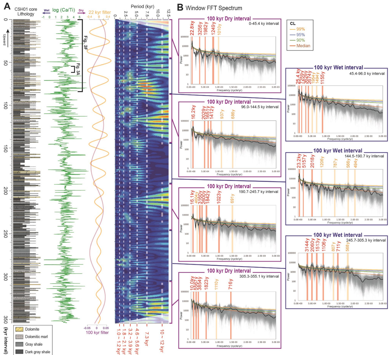
Figure 4. Decadal resolved changes in Ca/Ti ratios for a ~355-kyr interval. (A) Lithology, Ca/Ti ratios and wavelet analysis for a 29.6 m-thick (~355-kyr) interval of core CSH01 at 500 \mu\text{m} (~6 year) resolution using a XRF core scanner (Cox, Itrax). Amplitude modulation of 22-kyr filter (yellow; frequency: 4.5\text{e-}5 ; bandwidth: 1.0\text{e-}5 ) and 100-kyr filter (purple; frequency: 9.5\text{e-}6 ; bandwidth: 1.5\text{e-}6 ) are also shown. (B) Window FFT analyses of Ca/Ti variations for the drier interval and wetter interval of 100-kyr eccentricity minimum/maximum. Results of the Monte Carlo 1000 random runs concerning uncertainties of relative age estimations (Fig. S7) are shown as semitransparent grey lines. Significances of Fourier power spectrum are estimated for median values (black thick lines) only, assuming that subject power spectrum contains red-noise background signal. Reddish bars and numbers indicate significant spectral peaks above 99% CL. Yellowish bars and numbers indicate moderate spectral peaks above 90% CL. Window FFT analysis reveals pronounced but quasi-periodic millennial-scale periodicities centering on ~1010–1023, 1106–1155, 1206–1249, 1412–1513, 1823–2060, 3160–3854, 4604–5567, and ~7259 years, and less-pronounced centennial-scale periodicities of ~566–568, 686–716, and 787–810 years.
