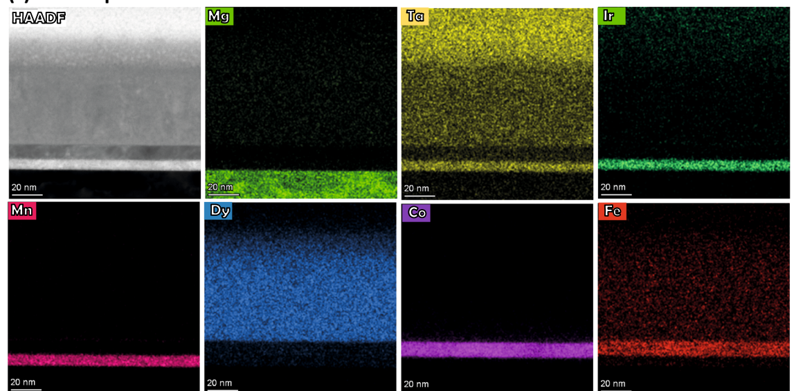
Figure 5. TEM and EDS for S3. (a) Cross-sectional TEM and HRTEM images of the specimen S3, show the sequence of layers on the MgO substrate. (b) FFT patterns of the area marked by the squares in (a) containing MgO, Mn 3 Ir, CoFe, and Dy. (c) EDS maps of the elements Mg, Ta, Ir, Mn, Dy, Co, and Fe in the layer stack show sharp interfaces along with the HAADF STEM image of the interfaces.
