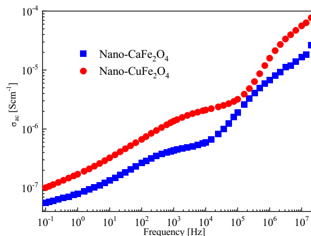
Figure 8. Frequency dependence of AC conductivity for \text{CaFe}_2\text{O}_4 and \text{CuFe}_2\text{O}_4 at room temperature.
