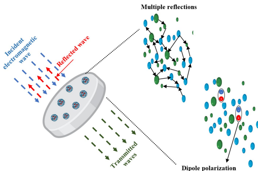
Figure 14. Schematic illustration of microwave absorption mechanism of coatings containing nano- \text{CaFe}_2\text{O}_4 and nano- \text{CuFe}_2\text{O}_4 .
