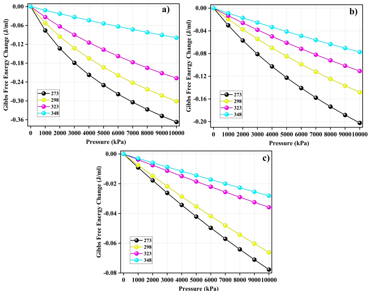
Figure 9. \Delta G values associated with (a) CO 2 , (b) CH 4 , and (c) N 2 adsorption on the surface of model coal-derived asphaltene at various temperatures.
