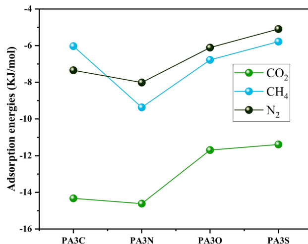
Figure 13. Examination of adsorption energies ( E_{ads} ) of CO 2 , CH 4 , and N 2 by the surface of asphaltene fragments.
