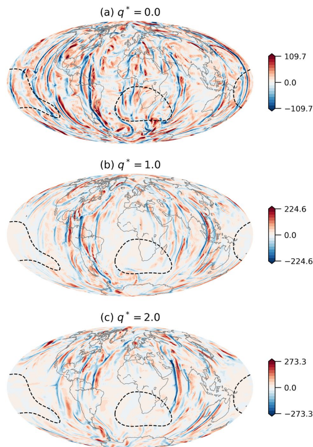
Figure 4. Non-dimensional radial velocity at the top of the shell ( r/r_o = 0.95 ) for dynamo models with (a) q^* = 0.0 , (b) q^* = 1.0 and (c) q^* = 2.0 . Dashed contours denote the regions where \delta q < \frac{1}{2} \delta q_{min} (see Fig. SM1). Note the different scales.
