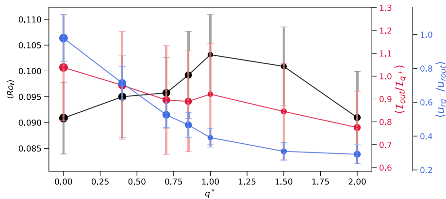
Figure 2. Diagnostics of the dynamo models vs. the outer boundary heat flux anomaly amplitude q^* . The local Rossby number Ro_\ell (13) is in black. The size of the symbols is proportional to the dipolarity f_{dip} (15). The ratio between the RMS azimuthal component of the inertial force at r/r_o = 0.95 outside/inside regions where \delta q > \frac{1}{2}\delta q_{max} (17–18) is in red. The ratio between the RMS radial velocity at r/r_o = 0.95 inside/outside regions where \delta q < \frac{1}{2}\delta q_{min} (19–20) is in blue. Error bars denote temporal variability.
