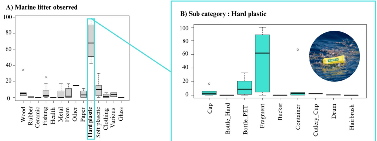
Fig. 2. Composition of marine litter observed from visual survey (A) Percentage abundance of marine litter by category, (B) percentage abundance of hard plastic subcategory.
