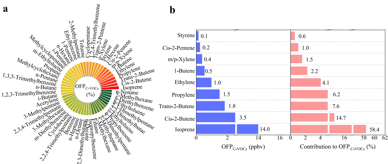
Fig. 4 \text{OFP}_{\text{C-VOCs}} of different species were calculated. a \text{OFP}_{\text{C-VOCs}} ( \text{OFP} calculated based on C-VOCs) importance ranking of all volatile organic compounds; b \text{OFP}_{\text{C-VOCs}} of the top nine reactive species and their percentage contributions to \text{OFP}_{\text{C-VOCs}} . This figure illustrates that reactive VOCs species should be valued for their participation in chemical reactions.
