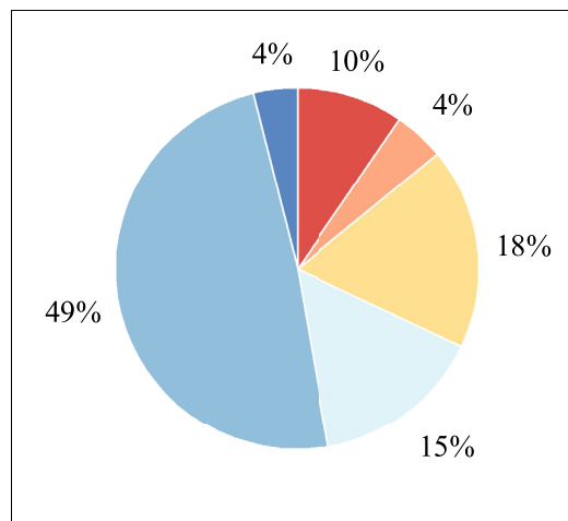
b Source contributions to OFP C-VOCs
