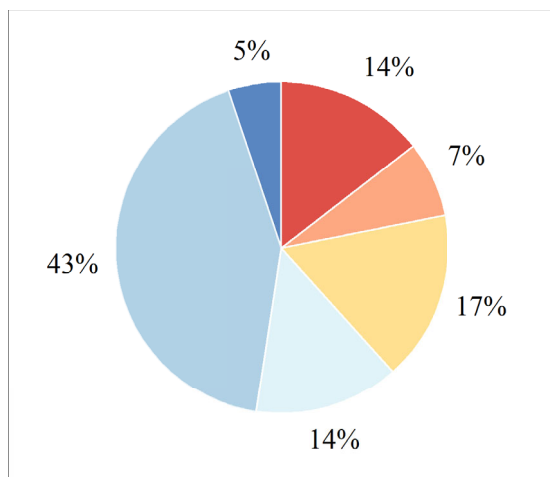
a Source contributions to consumed VOCs
