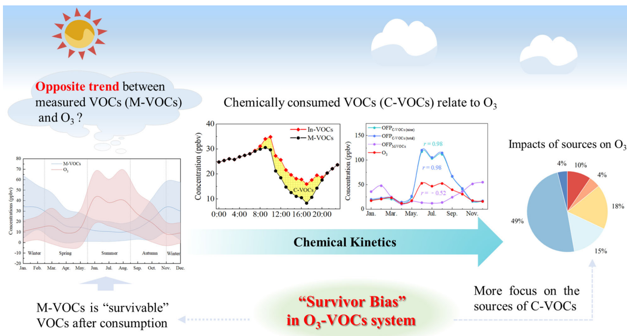
Fig. 6 Schematic diagram. This diagram explains the survivor bias for the O_3 -VOCs system. At the observation site, low-VOCs concentrations in summer correspond to high O_3 concentrations, while high VOCs concentrations in winter correspond to low O_3 concentrations. With the enhancement of photochemical reaction (in summer), VOCs with high reactivity will undergo photochemical reaction and participate in the accumulation of O_3 , resulting in less survivable M-VOCs. In contrast, a small number of VOCs were lost in winter, and the survivable M-VOCs gradually increased. Therefore, from the perspective of O_3 pollution control, we should focus more on the C-VOCs sources.
