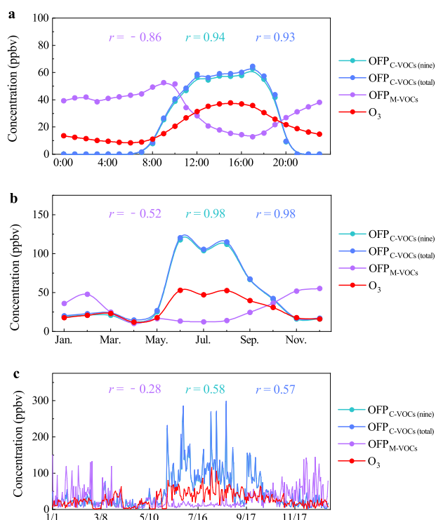
Fig. 3 The correlation of \text{OFP}_{\text{C-VOCs}} (nine), \text{OFP}_{\text{C-VOCs}} (total), \text{OFP}_{\text{M-VOCs}} and \text{O}_3 . Time series of a diurnal variation, b monthly concentration, and c daily concentration of ozone formation potential (OFP). Note that the \text{OFP}_{\text{C-VOCs}} (nine) and \text{OFP}_{\text{C-VOCs}} (total) ( \text{OFP} calculated based on the top nine or all C-VOCs) are higher than the observed \text{O}_3 especially in the summer. This may be because \text{OFP}_{\text{C-VOCs}} calculates maximum ozone formation potential, though \text{O}_3 consumption during the summer is substantial. Or due to the uncertainty of maximum incremental reactivity (MIR) when applied to the airshed conditions in 2018 in Tianjin, China. And the influence of physical processes (boundary layer height, etc.). Here, we mainly focus on the change trend of \text{OFP} and \text{O}_3 . The correlation between \text{OFP}_{\text{C-VOCs}} and \text{O}_3 is obviously higher than that between \text{OFP}_{\text{M-VOCs}} and \text{O}_3 , which further illustrates the important role of C-VOCs in \text{O}_3 formation.
