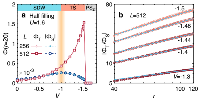
Fig. 4 Dominance of the triplet over singlet pairing in the half-filled TS phase. Here we show the data of U=1.6 . a Singlet and triplet pairing correlations at a fixed (long) distance r=20 . The yellow strip represents the transition point V_c \approx -1 from spin density wave (SDW) to triplet superconducting (TS) phase. b The calculated ratios |\Phi_T/\Phi_S| , plotted in a log-log scale, exhibit excellent agreement with the scaling r^{K_\rho-1} (blue solid lines).
