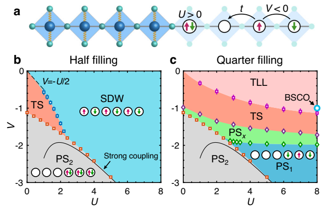
Fig. 1 Extended Hubbard model and phase diagrams. a illustrates the BSCO compound and corresponding extended t - U - V Hubbard model with NN hopping t , on-site repulsive U , and NN attractive V terms. b, c show the quantum phase diagrams of the EHM at half and quarter fillings, respectively. There are triplet superconducting (TS), spin density wave (SDW), and Tomonaga-Luttinger liquid (TLL) phases. There are also three phase separation phases with singly ( \text{PS}_1 ), doubly ( \text{PS}_2 ) or fractionally ( \text{PS}_x ) occupied clusters. The solid black lines represent the asymptotic phase boundary V = -\frac{U}{2} - \frac{8\ln 2}{30} in the strong coupling limit, and the dashed line for V = -U/2 in the weak coupling limit 30,54 . The blue circle in c represents the parameters U = 8 and V = -1 of the doped 1D cuprate chain BSCO 46 .
