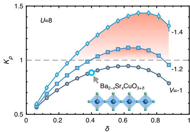
Fig. 6 Prediction for possible triplet superconducting phase in 1D cuprate chain. We show the Luttinger parameter K_\rho versus doping \delta for different attractive interactions V . In the highlighted regimes with K_\rho > 1 , there exists superconductivity phase for sufficiently strong attraction V and large doping \delta . The blue circle represents the cuprate \text{Ba}_{2-x}\text{Sr}_x\text{CuO}_{3+\delta} with the parameters V = -1 46 and \delta \approx 40\% , and a slight enhancement of the attraction can drive the compound to the triplet superconductive phase.
