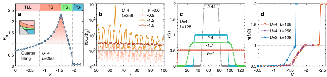
Fig. 5 Results of EHM at quarter filling. We show in a the mini phase diagram and Luttinger parameter K_\rho , and b accordingly the ratio between triplet and singlet pairings |\Phi_T/\Phi_S| that becomes greater than 1 in the emergent TS phase. The K_\rho results in the PS_x and PS_1 are computed within the clustered part (see Supplementary Note 3). c The charge distribution n(i) in TS ( V = -1 ), PS_x ( V = -1.7 ), PS_1 ( V = -2.4 ), and PS_2 ( V = -2.44 ) phases, respectively. d The charge densities n(L/2) measured at the center of the system are plotted versus V .
