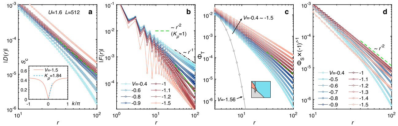
Fig. 3 Correlation functions of the half-filled EHM at U=1.6 . Here we show a density-density, b spin-spin, c the spin-triplet pairing, and d singlet pairing correlations, with various attractive interactions -1.5 \leq V \leq -0.4 . The color codes in the four panels are the same (following the representative color of each phase in Fig. 1b, as indicated by the legends in b , d ). The dashed green line represents \sim r^{-2} scaling that corresponds to K_\rho=1 , separating the exponential and power-law behaviors of various correlations in a , c , d . The dotted dash line \sim r^{-1} with exponent \alpha=1 in b represents long-distance scaling of the spin correlations in the SDW phase. The inset in a shows the charge structure factor at V=-1.5 , whose second-order polynomial fitting (dashed cyan line) results in a Luttinger parameter of K_\rho=1.84 .
