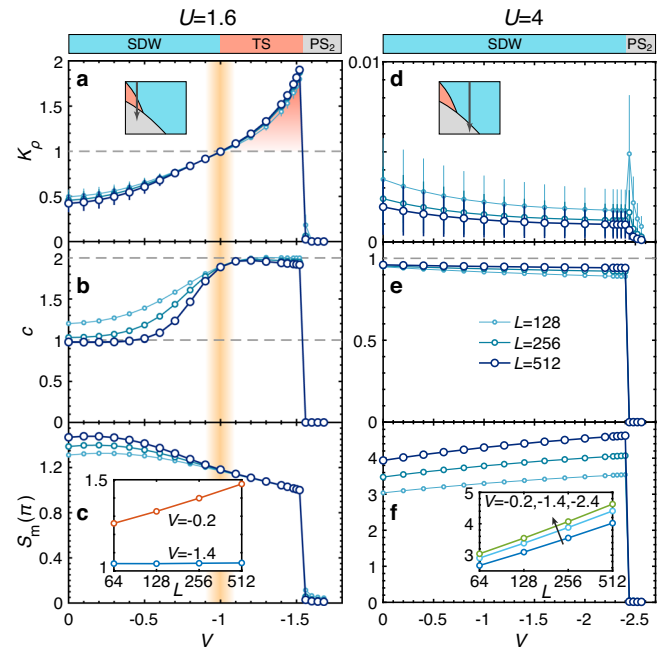
Fig. 2 Results of EHM at half filling. a–c are with on-site repulsion of U = 1.6 and d–f of U = 4 , with the corresponding mini phase diagrams also depicted. a, d show the results of the Luttinger parameter K_\rho , (b, e) are the results of central charge c determined from the entanglement entropy scalings, and c, f are the spin structure factors at \pi . Here the K_\rho results in a, d are obtained via the second-order polynomial fitting of S_c(k) in the small- k regime, with the error bars estimated by using different k -range for fitting (Supplementary Note 3). The insets in c, f show S_m(\pi) vs. L at various V s. a–c reveal the system undergoes a transition from spin density wave (SDW) to triplet superconducting (TS) phase at V_c \simeq -1 and then enters the phase separation (PS 2 ) regime for V < V_s \simeq -1.55 . d–f show no intermediate phase but a direct first-order transition from SDW to PS 2 at V_s \simeq -2.42 .
