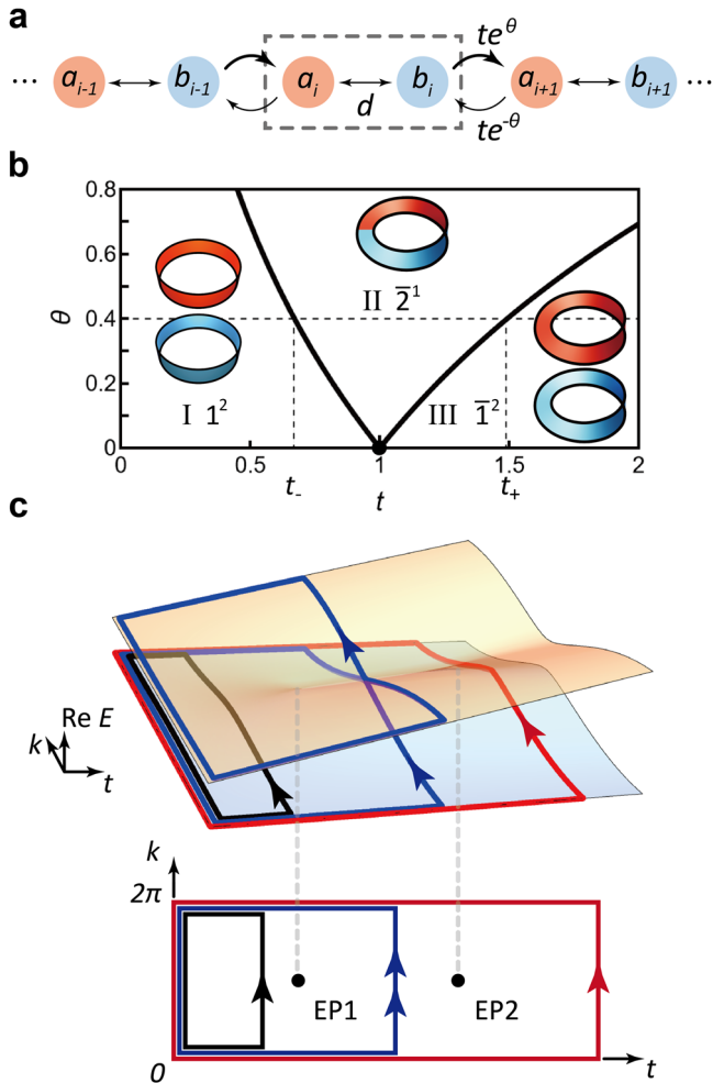
Fig. 2 | Two-band Su-Schrieffer-Heeger (SSH) model. a Non-Hermitian SSH model with non-reciprocal inter-unit-cell hopping. Intra-unit-cell hoppings are d and inter-unit-cell hoppings are te^{\theta} and te^{-\theta} . The dashed box denotes the unit cell. b Phase diagrams of the non-Hermitian SSH model. The black dot denotes a Dirac point, and the curved lines denote EPs. The 1^2 regime (I) is a trivial line-gapped regime of two trivial 1-cycle bands, the 2^1 regime (II) is a point-gapped regime of a 2-cycle non-separable band with a \pi Zak phase, and the 1^2 regime (III) is a line-gapped regime of two 1-cycle bands with \pi Zak phases. c The connection between the Zak phase of the one-dimensional SSH model and the EPs in parameter space, (t, k) space. Black, blue, and red paths respectively contain zero, one, and two EPs in (t, k) space, which correspond to 1^2 , 2^1 , and 1^2 phases.
