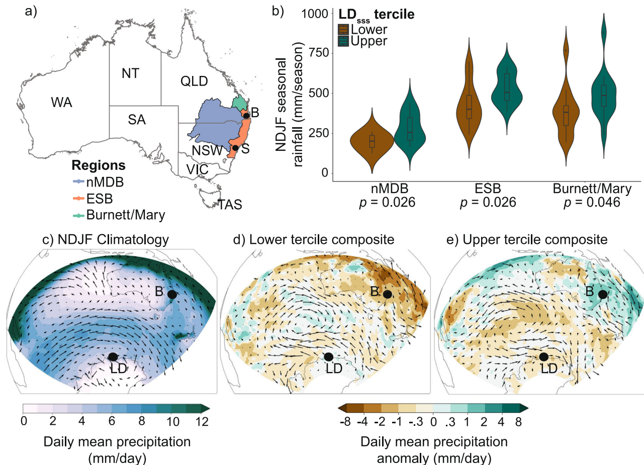
Fig. 1 Seasonal relationship between Law Dome summer sea salt ( LD_{ss} ) and eastern Australia rainfall over NDJF period from 1979/80 to 2015/16. a Australia map including locations of major east coast cities of Brisbane (B) and Sydney (S) and rainfall regions most strongly correlated to LD_{ss} 17,25 , incorporating key agricultural and urban water supply catchments; nMDB (blue) = northern Murray Darling Basin, ESB (orange) = eastern seaboard, and Burnett/Mary River catchment (green). b NDJF seasonal regional rainfall distributions over 1979/80 to 2015/16 for LD_{ss} upper ( LD_{ss} > 0.192 \log CI , n = 13 ) and lower ( LD_{ss} < 0.014 \log CI , n = 12 ) tertile years (>66%, <33%). Wilcoxon signed-rank test used to determine the significance (95%) of mean regional rainfall between LD_{ss} upper/lower tertile years over 1979/80–2015/16. Refer to Supplementary Fig. S1a for LD_{ss} timeseries split by tertile groups. c NDJF climatology over 1979/80–2015/16 (ERA-Interim 58 ) of daily total precipitation and surface winds (10 m) over study domain, including location of Brisbane (B) and Law Dome (LD). d NDJF composite conditions of daily total precipitation and surface wind (10 m) anomalies during LD_{ss} lower tertile years. e As e during LD_{ss} upper tertile years.
