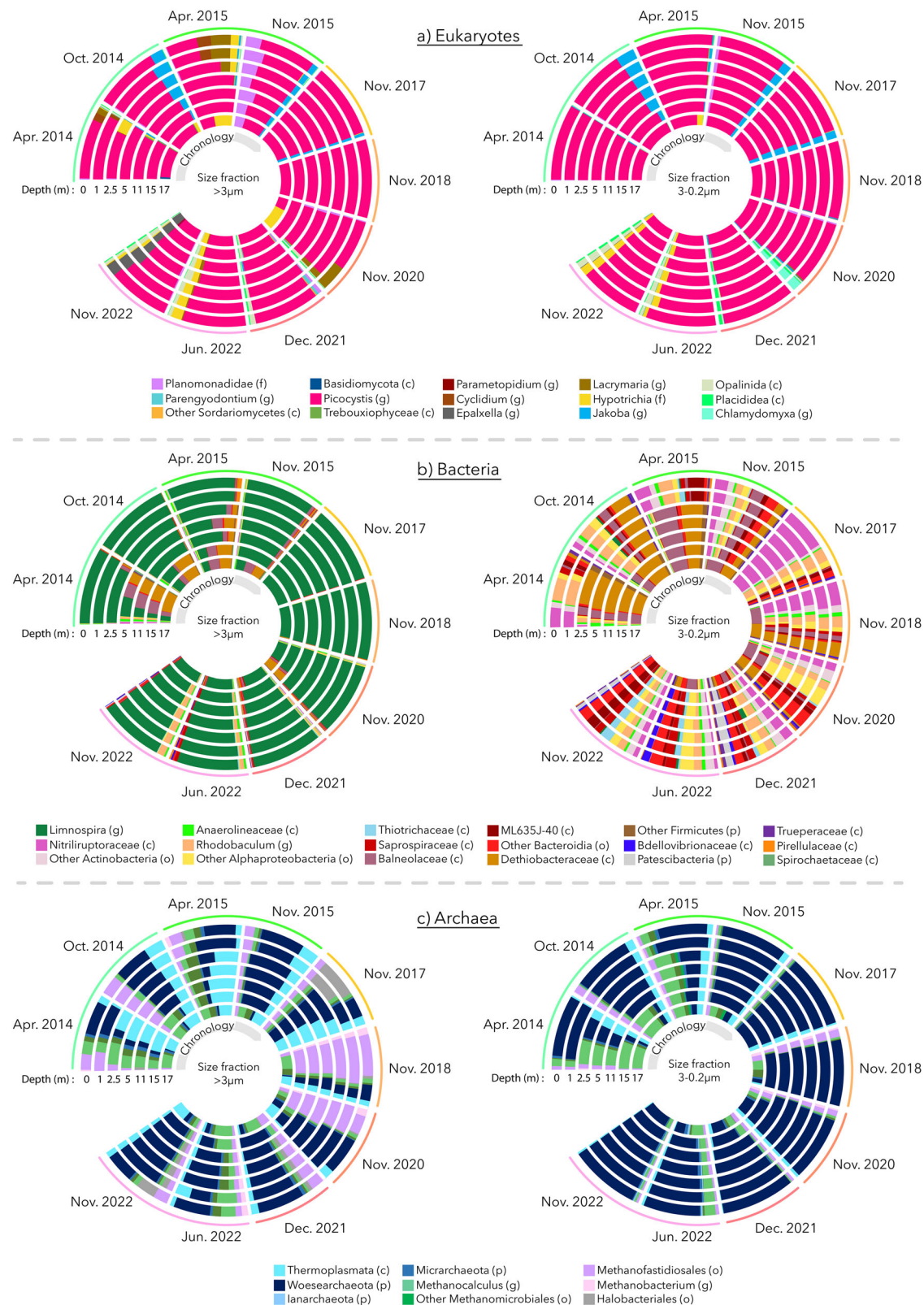
Fig. 2 | Interannual microbial community composition. a Microeukaryotic, b bacterial and c archaeal community structure in Lake Dziani Dzaha. Left graphs present the communities identified in >3 \mu\text{m} size fraction while right graphs show the communities detected in the 3-0.2 \mu\text{m} size fraction. Results are based on the relative proportions of 18S and 16S rRNA gene sequences. Apr. April, Oct. October,
