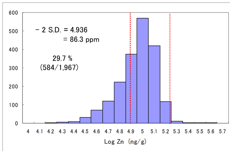
Figure 1 | Histogram of logarithmic zinc concentration in autistic children (N = 1,967). The histogram of scalp hair zinc concentrations for 1,967 children (1,553 males and 414 females) aged 0–15 years is shown in the logarithm. The numbers on the abscissa indicate the logarithms of scalp hair zinc concentrations ( \text{ng g}^{-1} ; ppb). The height of each rectangle represents the frequency in the class interval in logarithmic hair zinc level. Two dotted vertical lines represent the \pm 2 S.D. levels of the reference range of hair zinc concentrations.
