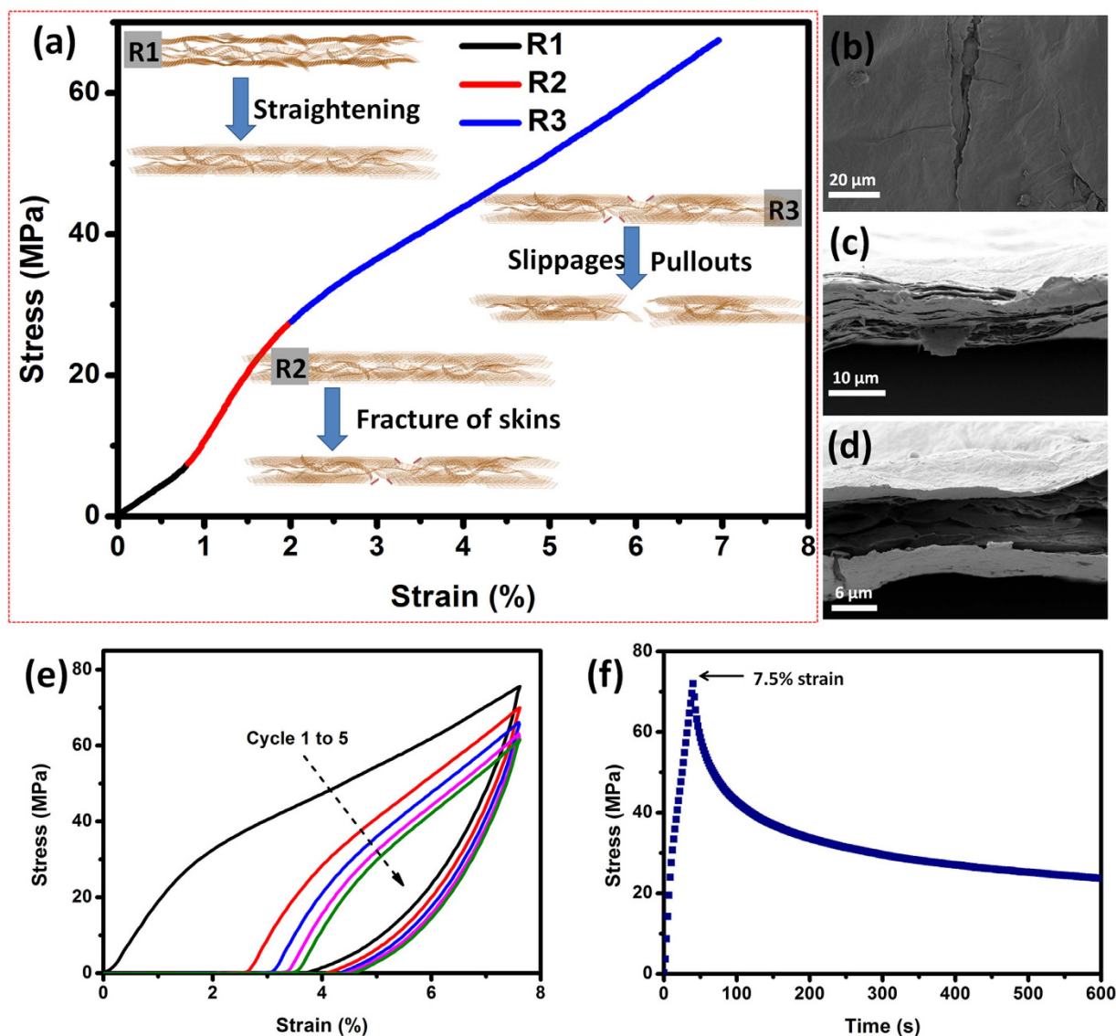
Figure 4. (a) A selected stress-strain curve of the 13.8-μm-thick C-GOF, demonstrating the fracture mechanism of the thick C-GOFs. SEM images of (b) the ruptured skins, and (c,d) irregular fracture sections of the stretched GOFs. (e) Loading-unloading cycling and (f) relaxation test of the 13.8-μm-thick C-GOF within 7.5% strain.
