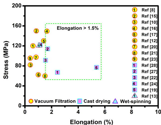
Figure 1. Statistical results of the mechanical properties of the reported pure GOs.
