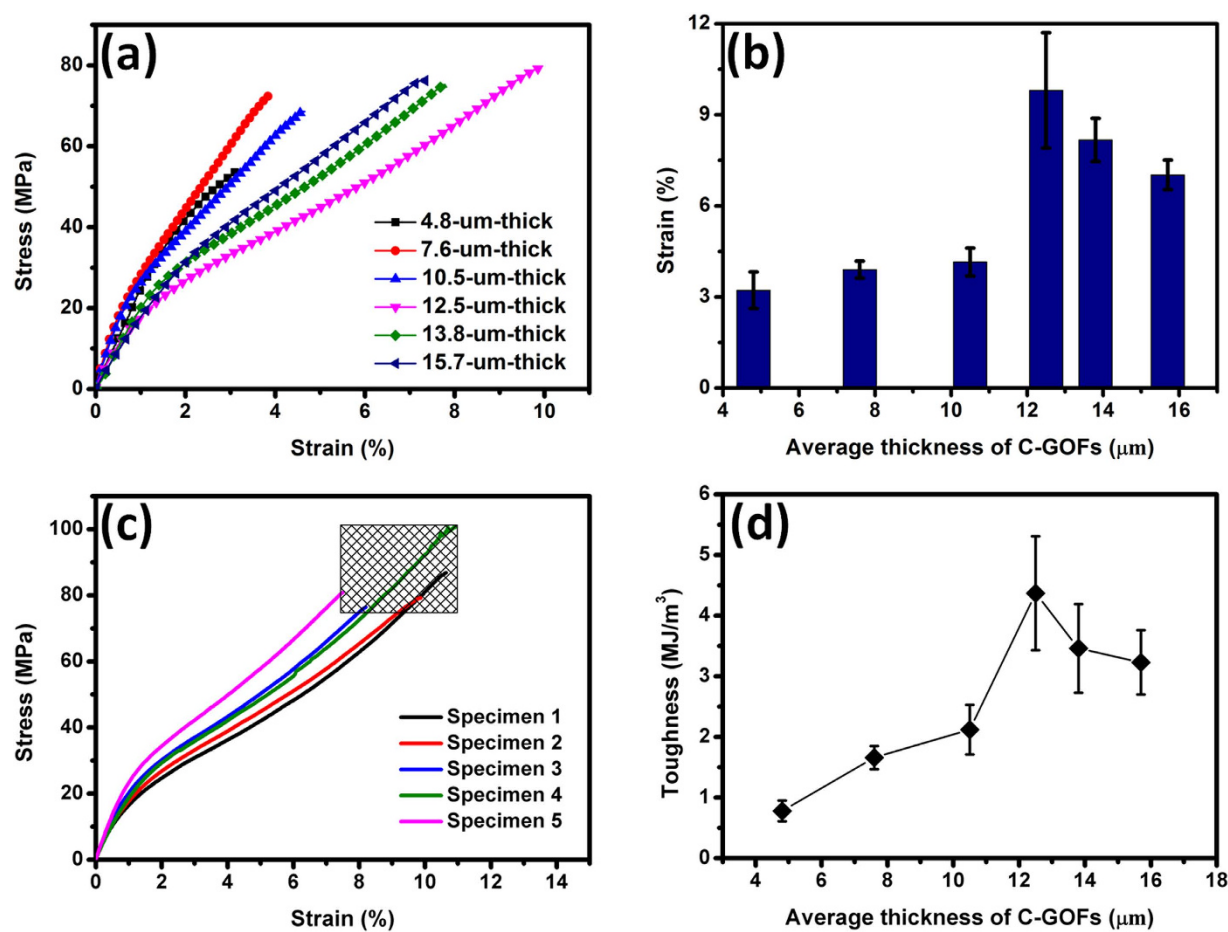
Figure 5. (a) Typical stress-strain curves and (b) average elongations of the C-GOFs in different thicknesses. (c) Five stress-strain curves of the 12.5-μm-thick C-GOF obtained from different specimens. (d) Thickness dependence of the toughness calculated from the stress-strain curves of C-GOFs.
