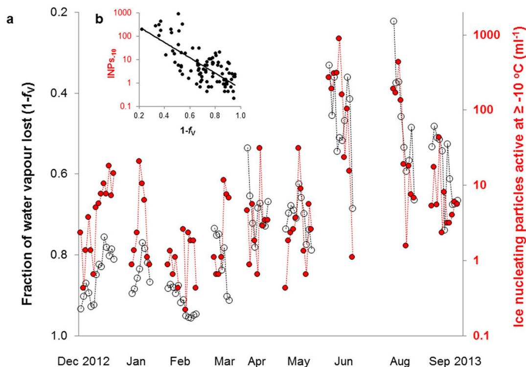
Figure 2. (a) Covariation over time of concentrations of INPs -10 in snow (red, log scale) and the estimated fraction of water vapour lost from an air mass prior to its arrival at the Jungfraujoch observatory (black). Time proceeds from left to right, intervals are not to scale. Each symbol signifies a snow sample with a median sampling duration of 2 hours. Each campaign (symbols connected by dotted lines, one campaign per month) lasted from 3 to 5 subsequent days. A total of 91 samples were collected between December 2012 and September 2013 (exception of July 2013 due to the lack of considerable precipitation events); (b) Relationship between INPs -10 and 1-f_v ; the function of the fitted exponential curve is reported in equation (1).
