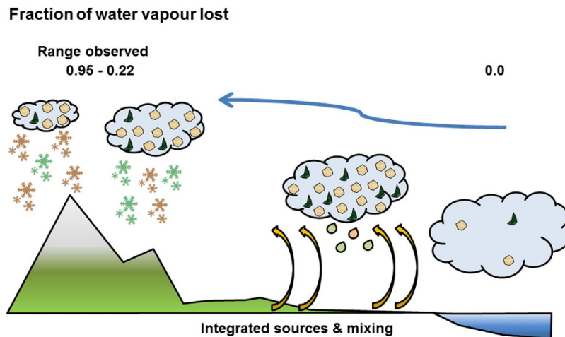
Figure 1. Relationship between the fraction of water vapour lost from a precipitating cloud (derived from stable isotope ratios in snow ( \delta^{18}\text{O} )) and ice nucleating particles (INPs, measured in snow). As the cloud precipitates, the progressive loss of water vapour (from right to left) is accompanied by a loss of INPs which have been uplifted from the sea and land surfaces (yellow arrows). INPs of biological origin (green half-moons) are activated at more moderate supercooling, hence typically earlier than inorganic INPs (brown hexagons). The values 0.22 and 0.95 correspond to the minimum and maximum fractions of water vapour lost that we observed at Jungfraujoch (drawn by E. Stopelli).
