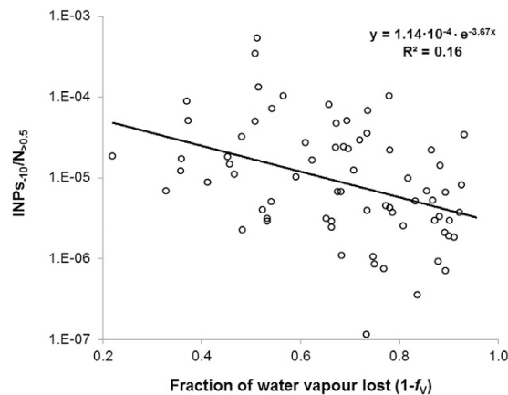
Figure 3. Ratio of \text{INPs}_{-10} to the total number of particles >0.5 \mu\text{m} ( N_{>0.5} , on log scale) as a function of the fraction of water vapour lost from the air mass prior to arrival at the observatory ( n = 71 , Spearman's r = -0.42 , p < 0.001 ).
