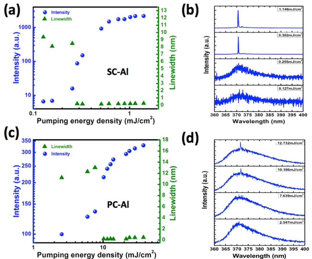
Figure 4. Emission intensity and linewidth as functions of the pumping energy density (a) for a nanolaser formed on the SC-Al/Al 2 O 3 template and (b) the corresponding emission spectrum. Emission intensity and linewidth as functions of the pumping energy density (c) for a nanolaser formed on the PC-Al/Al 2 O 3 template and (d) the corresponding emission spectrum. All the data are measured at 77 K.
