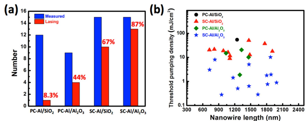
Figure 5. (a) Numbers of the measured and lasing nanowires corresponding to the four kinds of templates. (b) Threshold pumping energy density as a function of nanowire length for the four kinds of specimens. All the data are measured at 77 K.
