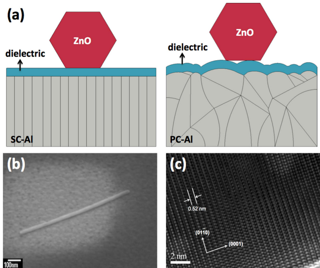
Figure 3. (a) Schematics of the ZnO nanowires formed on the tops of the single- and polycrystalline Al films with a dielectric spacer layer. (b) Scanning electron microscopy image of a ZnO plasmonic nanolaser. The length and hexagonal side length of the ZnO nanowire are 1 \mu\text{m} and 30 nm, respectively. (c) High-resolution transmission electron microscopy image of a ZnO nanowire taken along the [2\bar{1}\bar{1}0] direction.
