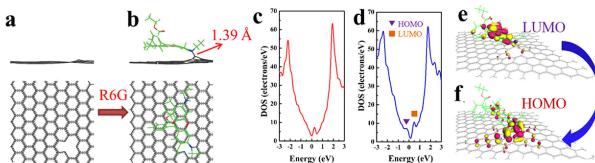
Figure 6. DFT calculation of the interaction of the R6G with the defect sites on graphene. Top and side views of graphene containing one defect (a). A single R6G molecule adsorbed on the graphene surface containing one defect, as simulated in a p(10 \times 10) cell. The graphene defect is the local adsorption site (b). DOS of the mono-vacancy in graphene (c) and R6G molecule adsorption (d). Calculated HOMO and LUMO profiles for the R6G/Graphene systems (e,f). Only one molecule per unit cell is performed per calculation.
