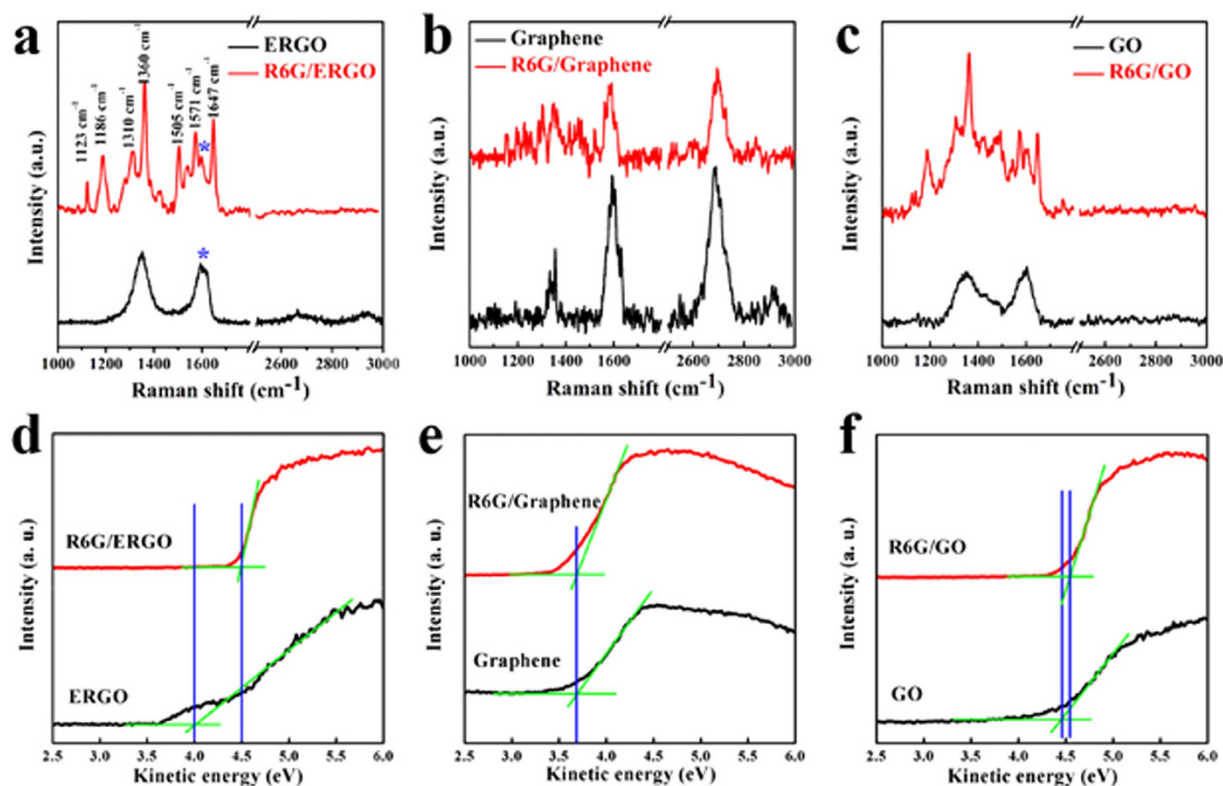
Figure 5. Raman spectra from R6G adsorption on the ERGO (a), graphene (b), and GO (c) substrates. The symbol “*” denotes the G-band of the ERGO. The UPS spectra of the ERGO (d), graphene (e), and GO (f) doped by R6G molecules at a concentration of 10^{-6} M.
