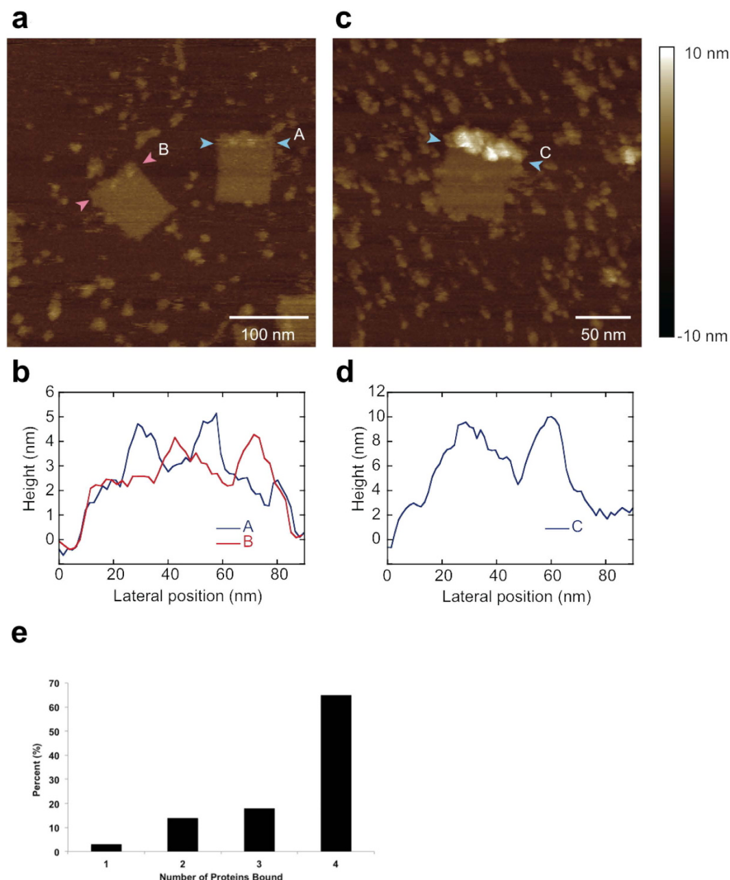
Figure 4. AFM images of AM-DNA origami in the presence of hLDH or PflDH. (a) Two modified DNA origamis in the presence of hLDH. Paths used for height profile measurements lie between the pink (“B”) and blue (“A”) arrowheads. (b) Height profile plot taken from the height profiles marked in (a). Each origami appears to have two distinct height maxima corresponding to positions of aptamers. (c) A modified DNA origami in the presence of PflDH. Paths used for height profile measurements lie between the blue (“C”) arrowheads. (d) Height profile plot taken from the height profiles shown in (c) show a large increase in height due to bound protein. (e) Analysis of PflDH binding to AM-DNA origami showing the percentage of measured AM-DNA origamis containing the indicated number of bound PflDH enzymes after incubation with an excess of enzyme ( n = 100 , mean = 3.5, std. dev. = 0.9).
