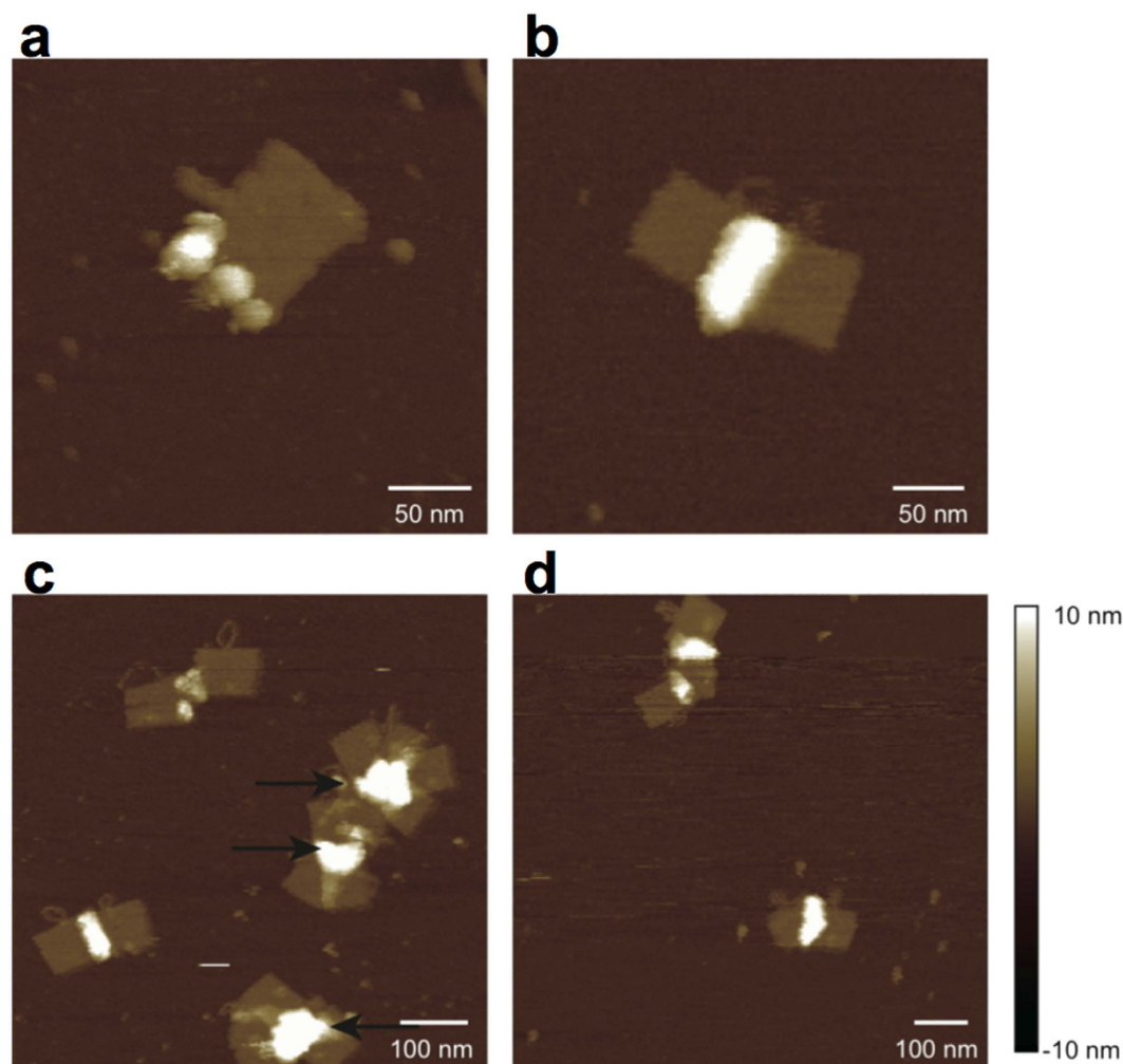
Figure 5. Effects of centrifugation and blood plasma. (a–c) Centrifugation of modified origamis constructed using 12 aptamers in the presence of Pfl DH resulted in a significant decrease in the amount of unbound protein while aptamer-bound protein remained. Centrifugation also promoted aggregation of origami structures, apparently via protein-protein interactions resulting in (b) dimerisation or (c) larger aggregates (indicated by arrows). (d) Presence of blood plasma has little effect on AM-DNA origami integrity or protein binding ability. Linear arrangements of Pfl DH are clearly visible and some aggregation occurs due to protein-protein interaction as a result of centrifugation.
