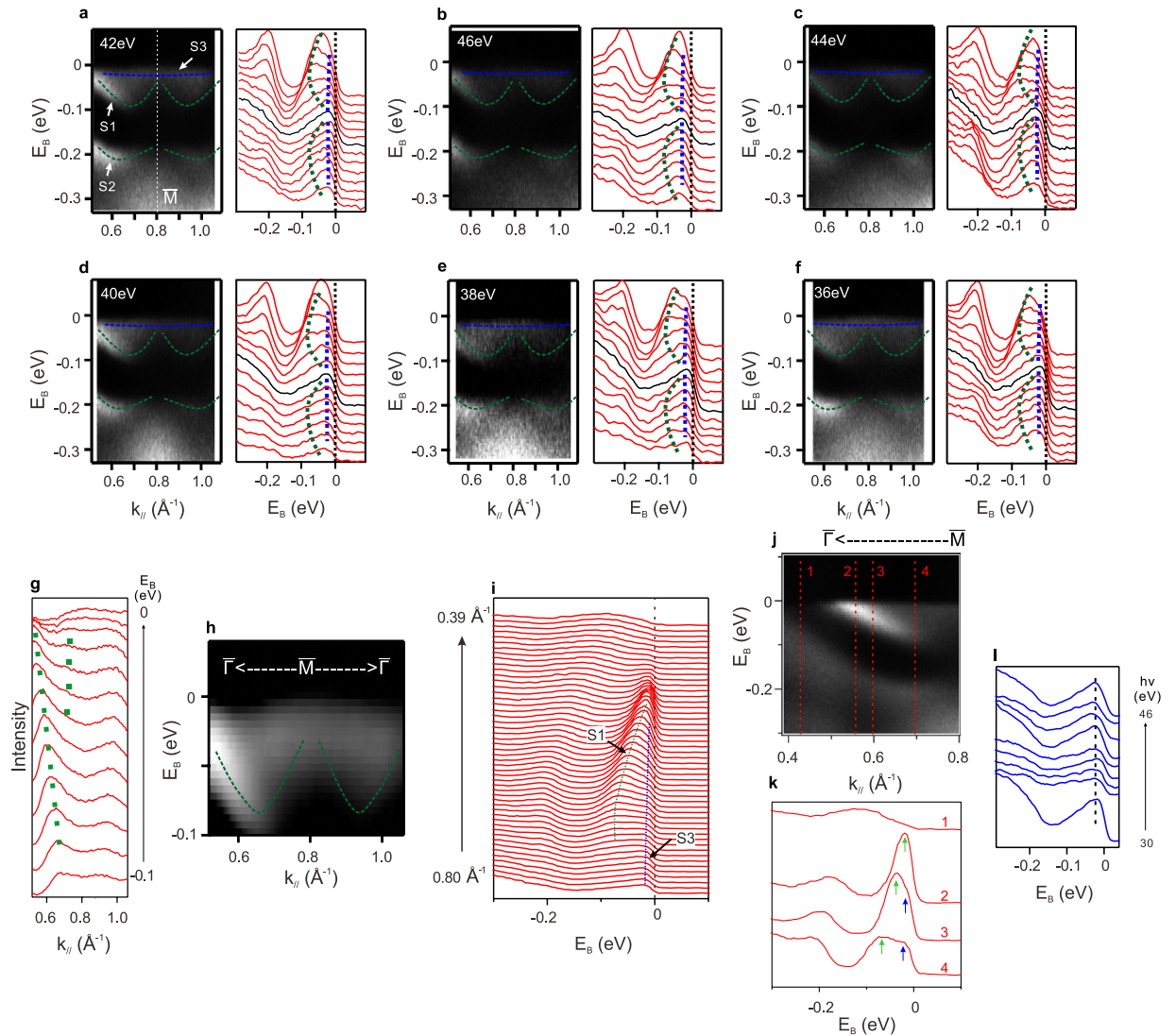
Figure 4. ARPES spectra near \bar{M} point. (a–f) ARPES spectra and corresponding EDCs of 30 nm Bi(111)/Bi 2 Te 3 film near \bar{M} point along \bar{\Gamma} – \bar{M} – \bar{\Gamma} (incident photon energy h\nu = 42, 46, 44, 40, 38 and 36 eV). Green and blue dashed lines are the guides for the S1, S2 and S3 bands. (g) MDCs near Fermi level extracted from (a). Green dotted lines mark MDC peaks of S1. (h) SDI plot of ARPES spectra ( h\nu = 30 eV) near \bar{M} point along \bar{\Gamma} – \bar{M} – \bar{\Gamma} direction. Green dashed line shows the possible dispersion of S1 band. (i) High resolution EDCs along \bar{M} – \bar{\Gamma} ( h\nu = 30 eV). Green and blue dotted lines mark EDC peaks of S1 and S3 bands. (j) The corresponding ARPES spectra of (i). (k) Four EDCs from (j). The momentum positions are indicated by the red lines in (j) ( k = 0.43 \text{ \AA}^{-1}, 0.56 \text{ \AA}^{-1}, 0.60 \text{ \AA}^{-1}, 0.70 \text{ \AA}^{-1} ). (l) EDCs at \bar{M} point as a function of the incident photon energy.
