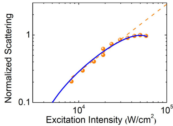
Figure 5. The scattering intensity dependence of 80-nm particles with 592-nm excitation. Orange circles are experimental points, orange dashed line shows the linear trend, and the blue curve is the fitting result with the quadratic equation.
