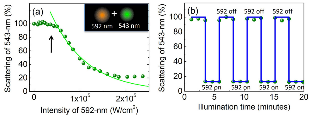
Figure 1. All-optical switching of scattering in a single gold nanoparticle. (a) The scattering intensity (normalized to the incident probe beam at \lambda = 543 nm with fixed intensity = 30 \text{ W/cm}^2 ) of an individual gold nanosphere as a function of the intensity of a control beam at \lambda = 592 nm. When the intensity of the control beam increases beyond 6 \times 10^4 \text{ W/cm}^2 , the scattering at \lambda = 543 nm starts to decrease. Green line is fitting for exponential decay with a threshold. (b) Demonstration of reversible switching of scattering for prolonged observation without bleaching (data were truncated for longer illumination time). Here the intensity of the \lambda = 592 nm control beam is 2 \times 10^5 \text{ W/cm}^2 .
