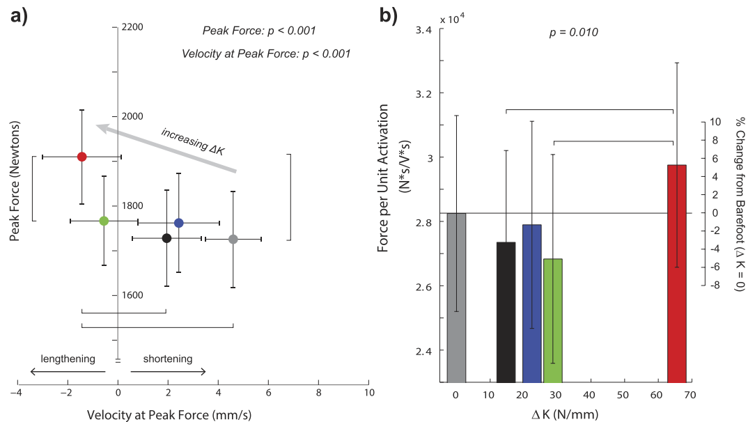
Figure 4. Slower fascicle shortening speed contributed to enhanced soleus force production. (a) Soleus peak force was plotted against fascicle velocity at the time of peak force ( N = 20 , mean \pm s.e.m). With added foot stiffness ( \Delta K ), there was a shift towards slower fascicle velocity at the time of peak plantar flexor force. At the greatest stiffness ( \Delta K = 65.6 N/mm), the soleus fascicle was actually lengthening during peak force production. P-values indicate the main effect of added foot stiffness, and significant pair-wise comparisons are denoted by the square brackets. (b) Force per unit activation was quantified as the ratio of integrated soleus force and integrated soleus activation during stance ( N = 19 , mean \pm s.e.m). Added foot stiffness increased the force per unit activation ( p = 0.010 ). The greatest added foot stiffness condition ( \Delta K = 65.6 N/mm) had greater force per unit activation compared to \Delta K = 14.8 N/mm and \Delta K = 28.7 N/mm (denoted by the square brackets).
