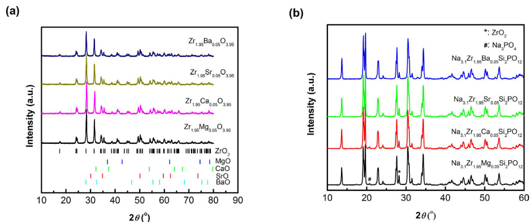
Figure 1. XRD patterns of (a) solid solutions of \text{ZrO}_2 and MO ( \text{M} = \text{Mg}, \text{Ca}, \text{Sr}, \text{Ba} ) after high energy ball milling for 2 h. (b) \text{Na}_{3.1}\text{Zr}_{1.95}\text{M}_{0.05}\text{Si}_2\text{PO}_{12} ( \text{M} = \text{Mg}, \text{Ca}, \text{Sr}, \text{Ba} ) sintered at 1260^\circ\text{C} for 16 h.
