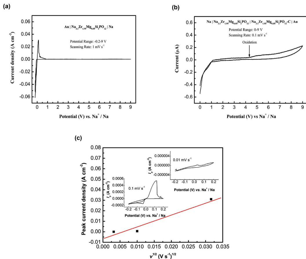
Figure 3. Cyclic voltammetry of Na 3.1 Zr 1.95 Mg 0.05 Si 2 PO 12 : (a) cyclic voltammetry of Au/Na 3.1 Zr 1.95 Mg 0.05 Si 2 PO 12 pellet/Na cell from -0.2 to 9 V at scan rate of 1 mV s -1 , (b) cyclic voltammetry of Au/Na 3.1 Zr 1.95 Mg 0.05 Si 2 PO 12 pellet/Na 3.1 Zr 1.95 Mg 0.05 Si 2 PO 12 -carbon/Na cell from 0 to 9 V at scan rate of 0.1 mV s -1 , and (c) Plot of peak current density vs. scan rate from the cyclic voltammetry. The inset is cyclic voltammetry curves at scan rate of 0.01 mV s -1 and 0.1 mV s -1 .
