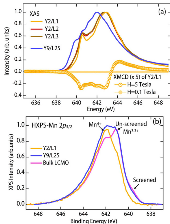
Figure 2. Heterostructuring effect on manganite layers. (a) Mn L_3 -edge x-ray absorption spectroscopy demonstrating that for up to 3 unit cells of LCMO, the Mn valence is fixed close to 4^+ rather than the expected 3.33^+ . For comparison, we show data from a thicker LCMO/YBCO superlattice (Y9/L25) with a nominal Mn valence of 3.33^+ . (b) HXPS spectra of Mn 2p_{3/2} , demonstrating that in Y9/L25 and bulk LCMO, Mn has nominal valence of 3.33^+ , whereas Mn in the Y2/L1 SL has nominal valence of 4^+ .
