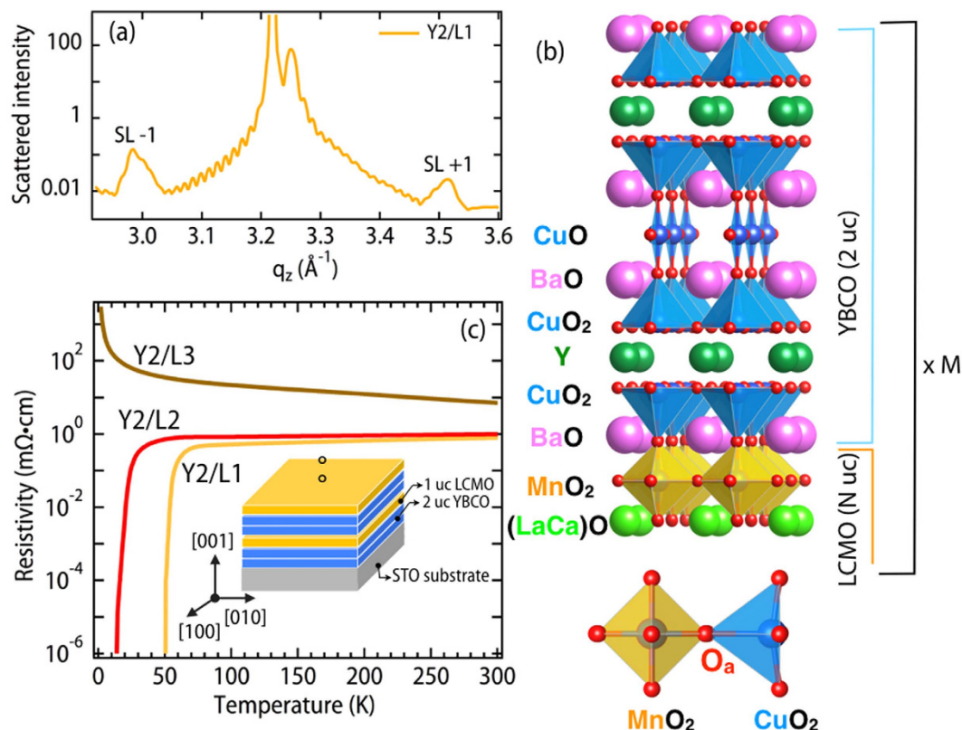
Figure 1. Crystal structure and electrical transport. (a) XRD scan for Y2/L1 sample showing clear thickness fringes and superlattice (SL) peaks. (b) The lattice structure consistent with the diffraction data of panel (a). (c) Electrical transport measurements showing a clear superconductor to insulator transition as a function of LCMO layer thickness. Inset shows growth sequence for Y2/L1 sample.
