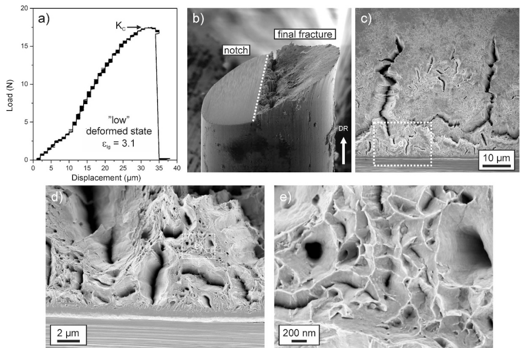
Figure 4. Mechanical test records and typical fractographs presenting significant fracture features in the perpendicular orientation of the low deformed state ( \epsilon_{lg} = 3.1 ). (a) Load-displacement curve showing pronounced plasticity before failure. The change in the slope in the elastic regime after about 10 \mu\text{m} is due to an adjustment of the unloaded specimen into the tensile direction. (b) Side-view onto a broken sample depicting the pre-notch and the final fracture surface. Sample diameter is 120 \mu\text{m} . (c) Typical fractograph looking parallel to the drawing direction. Several large delamination can be observed, which seem to have no specific alignment. (d) Enlarged view of inset in (c) demonstrating a large variety of smaller delaminations adjacent to the pre-crack. (e) Magnified view of detail shown in (d). Between the delaminations typical features of ductile fracture with dimples in the range of several hundred of nanometers can be seen.
