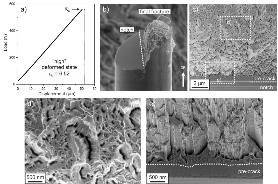
Figure 5. Mechanical test records and typical fractographs presenting significant fracture features in the perpendicular orientation of the high deformed state ( \epsilon_{lg} = 6.52 ). (a) Load-displacement curve with pure linear-elastic behavior before failure. (b) Side-view onto a broken sample with indicated pre-notch and final fracture surface. Sample diameter is 24\mu\text{m} . (c) Typical fractograph recorded looking parallel to the drawing direction at low magnifications. (d) Magnification of detail indicated in (c) with ductile fracture features. (e) Inclined view onto the transition from pre-crack to final fracture that shows various delaminations before the crack deflects and propagates into the drawing direction. The view is about 30^\circ inclined to the drawing direction to give a better view onto the transition zone with its delaminations and the final crack deflection.
