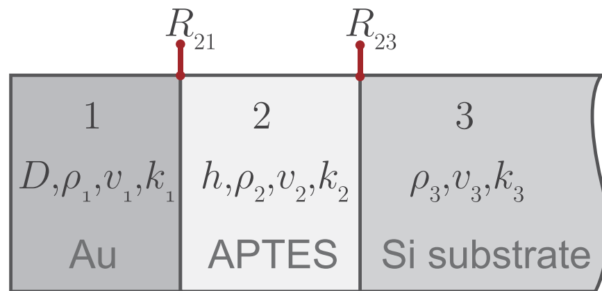
Figure 5. Schematic of the layer system and respective definitions for the theoretical modelling.
