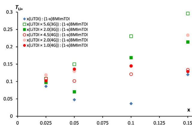
Figure 3. Dependence of lithium cation transference number dependence on LiTDI content in LiTDI–BMImTDI–glyme mixtures at room temperature for (a). Triglyme, (b). Tetraglyme. All values were averaged over at least three samples.
