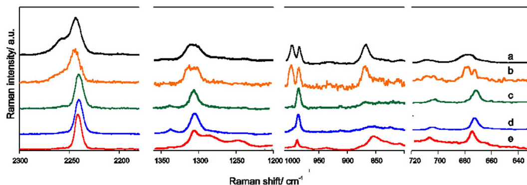
Figure 4. Raman spectra of samples: (a) molten LiTDI-4G. (b) 0.1[LiTDI-4.5(4G)]:0.9BImTDI (subtraction spectrum), (c) 0.1[LiTDI-2.0(4G)]:0.9BImTDI (subtraction spectrum), (d) 0.1[LiTDI-1.0(4G)]:0.9BImTDI (subtraction spectrum), (e) BImTDI.
