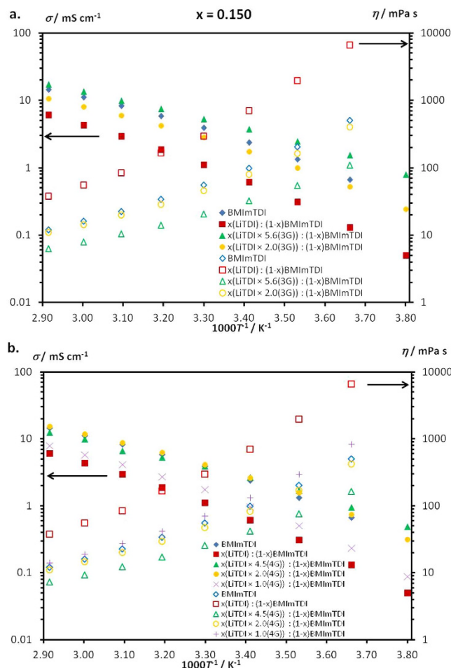
Figure 2. Inverse temperature dependence ( 1000T^{-1} ) of ionic conductivity and viscosity for LiTDI–BMImTDI–glyme systems for mole fraction of salt x = 0.150 containing (a). triglyme (3G), (b). tetraglyme (4G). The results of two-component systems were added for comparison 8 . Temperature 20 °C corresponds to the value 3.41 on the x axis and temperature 70 °C corresponds to the value 2.91 on the x axis.
