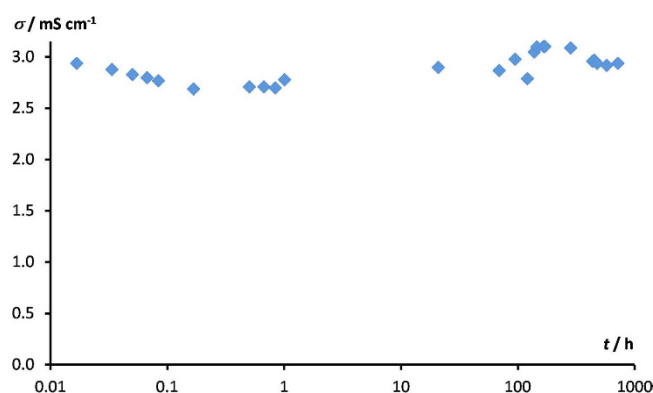
Figure 5. Time dependence of ionic conductivity for 0.15[LiTDI-4.5(4G)]:0.85BImTDI system at room temperature.
