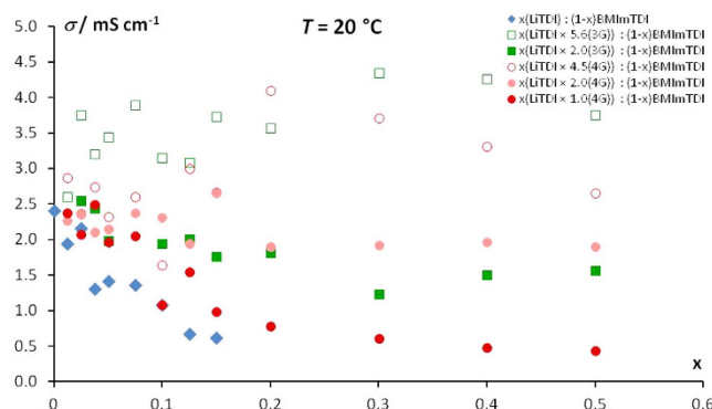
Figure 1. Dependence of ionic conductivity at 20 °C on LiTDI content in BMImTDI with the addition of triglyme with molar ratio of 1:2 and 1:5.6 and tetraglyme with molar ratio of 1:1, 1:2 and 1:4.5; the results of two-component systems were added for comparison 8 .
