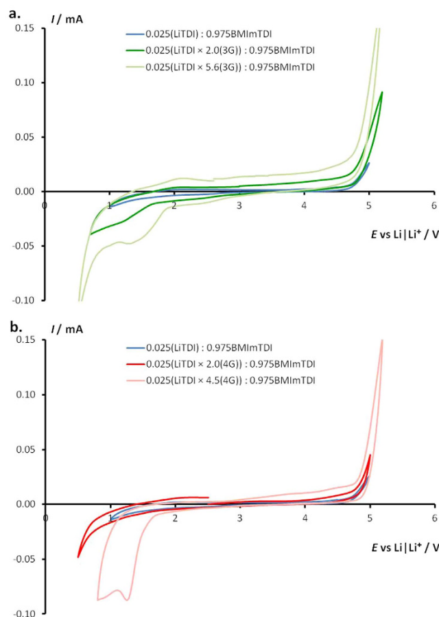
Figure 6. Cyclic voltammogram (CV) of ternary systems 0.025[\text{LiTDI} \cdot \gamma(\text{glyme})] : 0.975\text{BImTDI} at room temperature containing (a). triglyme ( \gamma = 2.0 or 5.6 ), (b). tetraglyme ( \gamma = 2.0 or 4.5 ). Metallic lithium acts both counter and reference electrodes. The scan rate was 1 \text{ mV s}^{-1} .
