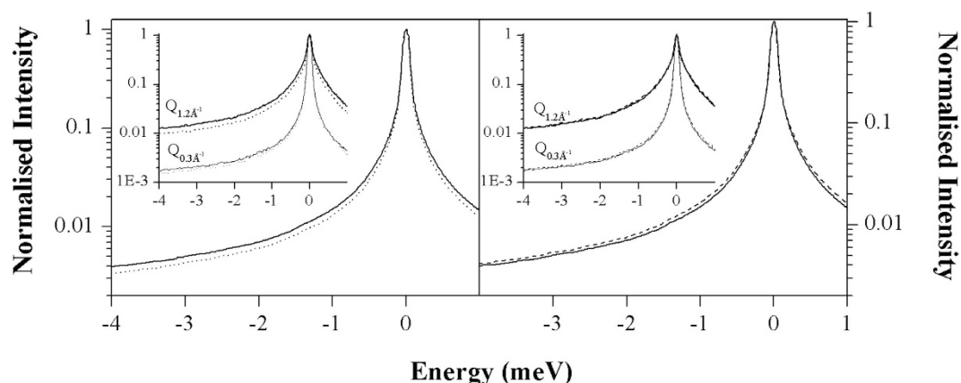
Figure 1. Quasi-elastic neutron scattering intensities, at 298 K, binned over the whole wave-vector range accessible on the IN5 spectrometer ( 0.2\text{--}2\text{ Å}^{-1} ) and normalized to unity. Left panel: H30S-3 M NaCl (solid line) and H50S-3 M NaCl (dotted line), Right panel: -H30S -3 M NaCl (solid line) and H30S-3 M KCl (dashed line). Insets: same spectra at reference Q=0.3\text{ Å}^{-1} (fluctuation amplitudes > 20\text{ Å} ) and Q=1.2\text{ Å}^{-1} (amplitudes \sim 5\text{ Å} ). A broader intensity distribution indicates scattering from faster motions (see text).
