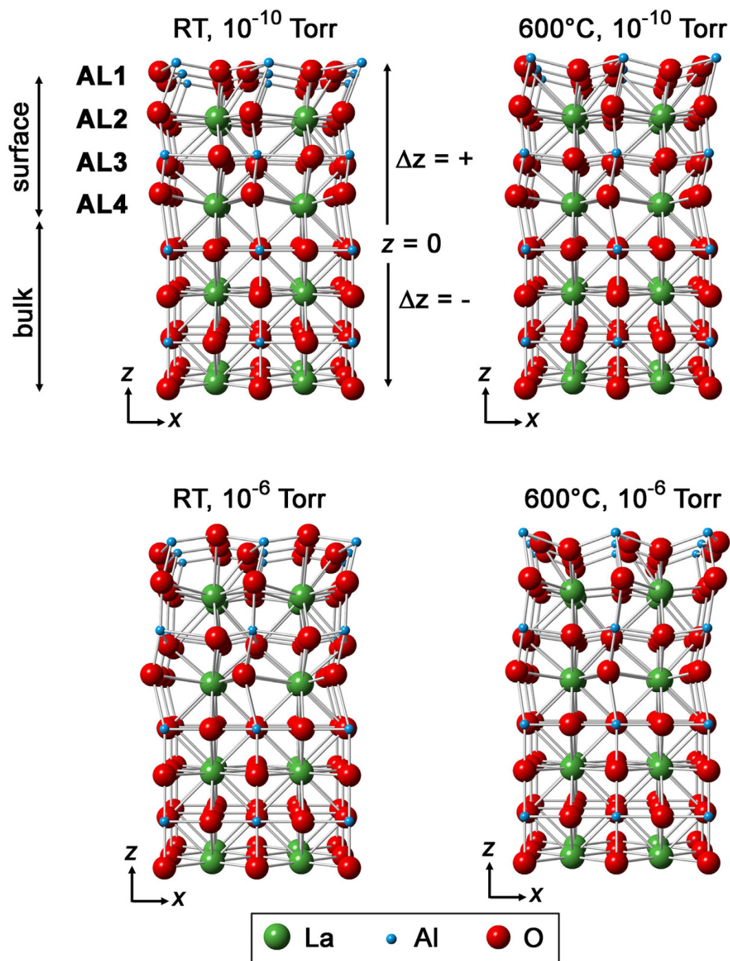
Figure 6. Structural representation projected along [010] comprises the bulk and surface species at different conditions whilst the [100] projection is presented in Fig. S8.
