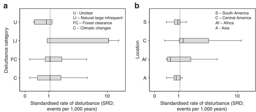
Figure 4 | Composite figure showing the standardized rate of disturbance (SRD) of different disturbance categories and locations. Box plots displaying the relationship between the SRD and (a) different grouped disturbance categories and (b) geographical location groups. (See Fig. 2 legend for details on notation and sample sizes). The SRD is plotted on a logarithmic scale to accommodate the variability in the data set. The vertical line in a and b represents the median SRD for the entire data set, that is, 1.072 disturbance events per 1,000 years. Shaded areas on a and b represent the interquartile range and the whisker lines the 95% confidence intervals for each category.
