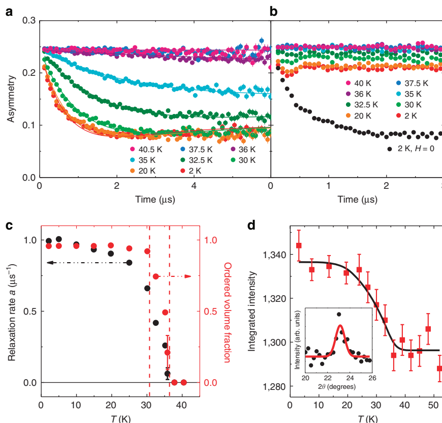
Figure 4 | Muon spin relaxation and neutron diffraction. (a) Time dependence of the asymmetry in H = 0 , fit with equation (1) (solid lines). (b) A small applied longitudinal field \mu_0 H = 0.01 T eliminates the relaxation response. For comparison, the H = 0 T = 2 K asymmetry is shown in black circles. (c) Relaxation rate a (black circles, left) and volume fraction (red circles, right) as a function temperature ( H = 0 ). (d) Integrated intensity of the (0, \pi/b, 0) TiAu magnetic Bragg peak as a function of temperature with mean-field fit ( T_N = 36 \pm 2 K, black curve). Inset: net counts normalized for 2 min. counting time between 2.5 and 60 K, showing the (0, \pi/b, 0) magnetic peak fit with a resolution-limited Gaussian (red line). Uncertainties are statistical in origin and represent one standard deviation.
