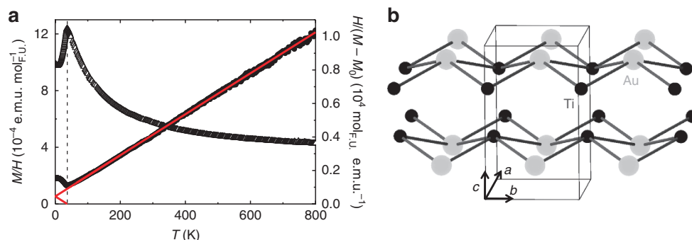
Figure 1 | Temperature-dependent magnetization of TiAu. (a) Left axis: zero-field-cooled magnetic susceptibility as a function of temperature for \mu_0 H = 0.1 T applied field ( 1 \text{ e.m.u.} = 10 \text{ A cm}^{-2} ). Right axis: inverse susceptibility H/M along with a Curie–Weiss-like fit (solid line), with \theta \approx -37 K (marked by a dashed line). (b) The crystal structure of TiAu with Ti (small) and Au (large) atoms, and the orthorhombic unit cell outlined in thin black lines. The arrows identify the crystallographic directions, marked by a , b and c axes.
