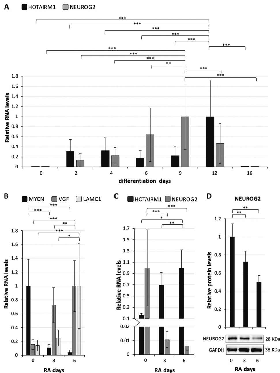
Fig. 1 HOTAIRM1 and NEUROG2 expression are inversely correlated during neuronal differentiation. a qRT-PCR analysis of HOTAIRM1 and NEUROG2 expression along differentiation of iPSCs into ventral spinal cord lineages. Differentiation days are reported on the x-axis. Expression levels are relative to ATP5O and expression peaks are set as 1. N = 1, 2 or 3, depending on the sample. **P \leq 0.0021 , ***P \leq 0.0002 . b qRT-PCR analysis of mRNAs coding for MYCN (proliferative marker), VGF (neuropeptide precursor) and LAMC1 (neurite-promoting factor) along neuronal differentiation of SH-SY5Y cells. Days of RA treatment are reported on the x-axis. Expression levels are relative to GAPDH , expression peaks are set as 1. N = 3 , *P \leq 0.05 , **P \leq 0.01 , ***P \leq 0.001 . c qRT-PCR analysis of HOTAIRM1 and NEUROG2 expression along neuronal differentiation of SH-SY5Y cells. Broken axis-histogram allows to appreciate low values. Details as in (b). N = 2 or 3, depending on the target. *P \leq 0.05 , **P \leq 0.01 , ***P \leq 0.001 . d Immunoblot analysis of NEUROG2 along neuronal differentiation of SH-SY5Y cells. Days of RA treatment are reported below each lane. In the histogram, NEUROG2 levels are relative to GAPDH. N = 3 , **P \leq 0.01 .
