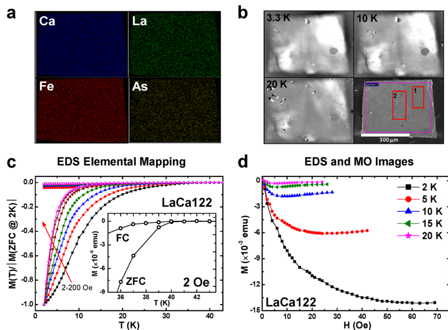
Fig. 2 EDS elemental mapping and superconducting magnetization properties for La-doped \text{CaFe}_2\text{As}_2 . a The EDS elemental mapping for LaCa122 shows that all of the elements in the crystal are homogeneously distributed. b However, the magneto-optical (MO) images show localized strong-SC regions. The MO images at 3.3, 10, and 20 K are measured in the remanent states, and the bright regions indicate strong-SC regions, where the high- T_c phase is dominant. The EDS results in regions 1 and 2 are not different despite the presence of very different SC states, implying that nanoscale inhomogeneity is important. c Zero-field-cooled (ZFC) and field-cooled (FC) dc magnetization ( M ) data for applied magnetic fields of 2, 5, 10, 20, 50, 100, and 200 Oe. Here, M(T) is normalized to the ZFC M value at 2 K. As shown in the inset, a clear separation between the ZFC and FC data at 2 Oe is observed at temperatures below 40 K, but the SC volume fraction at high temperatures is easily suppressed by small magnetic fields. d The magnetic field dependence of M at temperatures of 2, 5, 10, 15, and 20 K. The rapid suppression of M(H) at high temperatures implies a small volume fraction for the high- T_c phase in LaCa122
