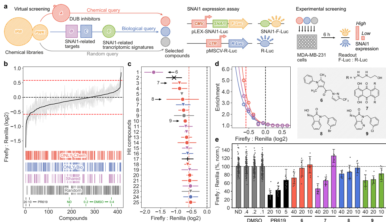
Fig. 4 Library enrichment to identify Snail1 inhibitors. a Scheme of the methodology. Two compound libraries are screened (IRB and PWK). A chemical query is done by looking for similarities with known DUB inhibitors. A biological query is done by looking for transcriptional (D1) and network-based (C3-5) signature matchings with Snail1-relevant targets. Random molecules are selected to estimate the background hit-rate. A Snail1 expression assay based on Firefly:Renilla luciferase ratios are used to screen candidate compounds. b Library enrichment quantification showing the effects of compounds selected by chemical (red), biological (blue), shared between both (magenta), and random (gray) queries, as well as the positive (PR-619) and negative (DMSO) controls. c Detail of the top 25 hit compounds. d Fold enrichment of compounds selected by chemical (red), biological (blue), and shared (magenta) queries with respect to random picks, based on their capacity to modulate Snail1 levels (Firefly:Renilla assay). Median \pm MAD ( n = 4 ). e MDA-MB-231 cells stably expressing luciferase constructs were treated for 6 h with the indicated compounds, at different doses. Firefly:Renilla ratios were normalized with the corresponding concentration of vehicle (DMSO). Mean \pm SD of 2 independent experiments, each of them including 4 replicas, are shown.
