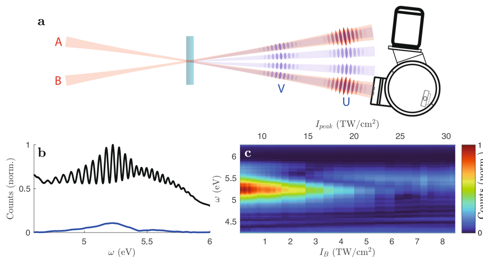
Fig. 2 | Experiment. a Two fundamental beams (red) are focused into a crystal (crossing angle \alpha = 1.1^\circ , beam waist 120\ \mu\text{m} ). Beams in the DUV (blue) are emitted from the laser-induced grating both collinearly to the fundamental beams and in the interstitial space. The wavefronts of the fundamental pulses A and B, which originate by beam splitting of one laser pulse, are highlighted in red. Cross-phase modulation scans (XPMS) are used for experimental pulse retrieval 23 and indicate a center wavelength of 700 nm and a pulse duration of 8 fs. The DUV beams contain two pulses (wavefronts highlighted in blue), of which the front pulses travel at the
