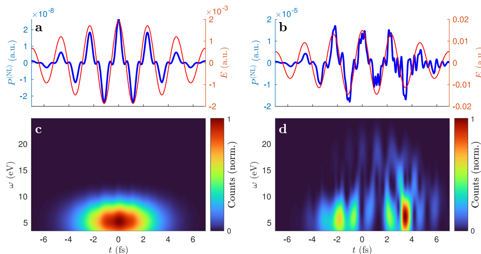
Fig. 6 | The nonlinear polarization response in time domain. P^{(NL)} is calculated using the SBEs with Bloch electron motion at 0.2 TW/cm 2 (a) and (c) and at 4 TW/cm 2 (b) and (d). The blue lines in a and b show P^{(NL)} , the generating field is
