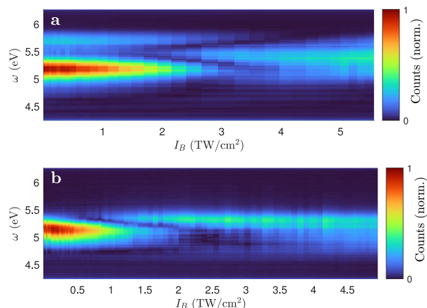
Fig. 3 | Comparison with other crystals. The Fourier filtered spectrum I_f(\omega) as a function of intensity as in Fig. 2 but for \text{Al}_2\text{O}_3(110) ( a ) and \text{MgO}(100) ( b ).
