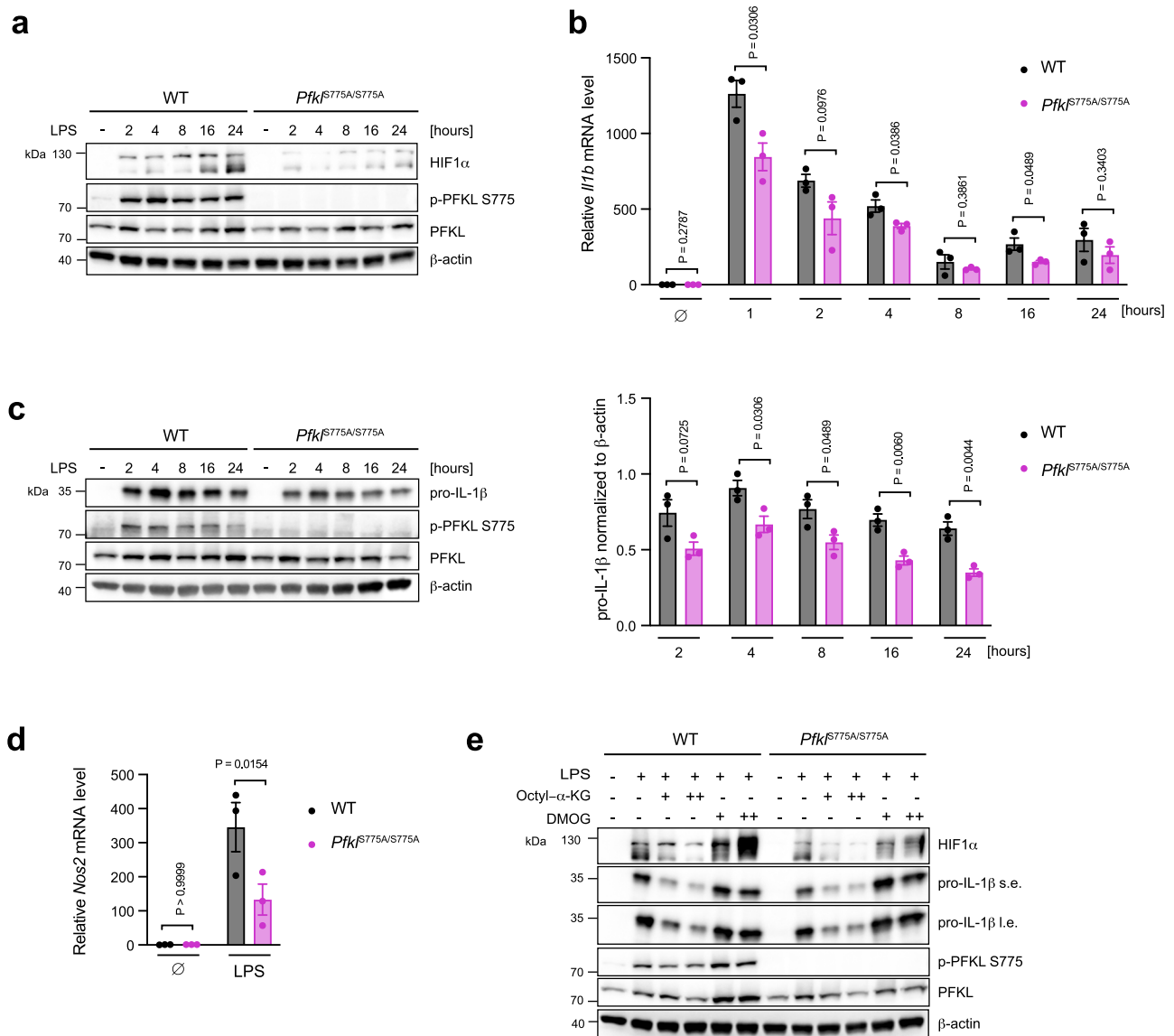
Fig. 6 | PFKL Ser775 phosphorylation is required for LPS-induced HIF1α and IL-1β production. a mBMDM from WT and Pfkf S775A/S775A mice were stimulated with LPS (200 ng/ml) for the indicated time periods. Indicated proteins were analyzed by western blot. β-actin was used as a loading control. b LPS-induced Il1b mRNA levels in WT and Pfkf S775A/S775A mBMDM were measured by qPCR and normalized to Actb mRNA levels. Data are presented as mean ± SEM ( n = 3 ), statistics indicate unpaired two-tailed student's t -test. c mBMDM from WT and Pfkf S775A/S775A mice were stimulated with LPS for the indicated time periods. Indicated proteins were analyzed by western blot (left panel). LPS-induced pro-IL-1β were quantified by normalization to β-actin at indicated time points (right panel). Data are presented as mean ± SEM ( n = 3 ), statistics indicate unpaired two-tailed student's t -test. d mBMDM from WT
