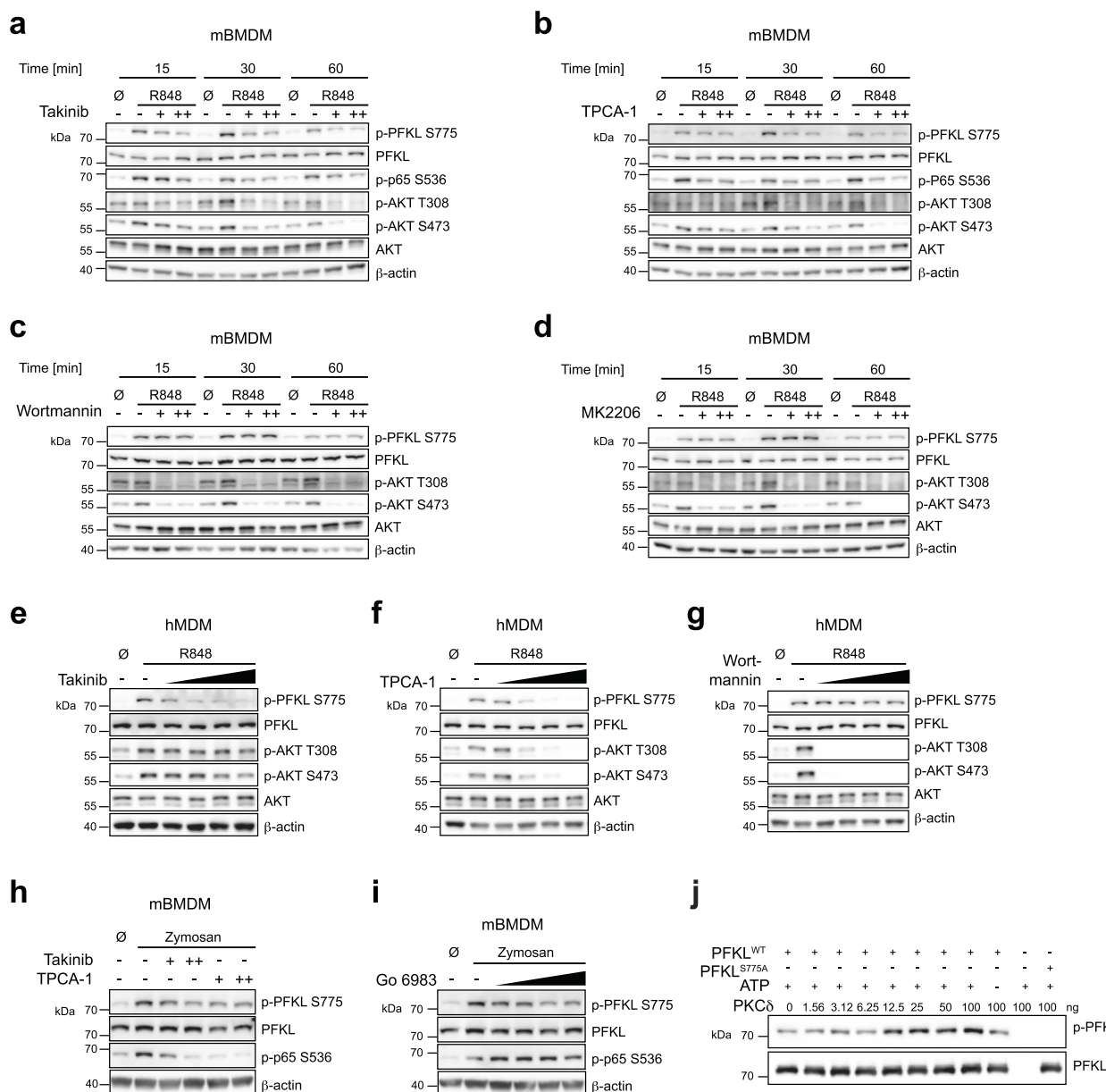
Fig. 2 | The IKK complex and PKC function in PFKL Ser775 phosphorylation. Immunoblot analysis of indicated proteins. mBMDM were pretreated with DMSO, Takinib (+, 50 \mu M; ++, 100 \mu M) (a), TPCA-1 (+, 5 \mu M; ++, 10 \mu M) (b), Wortmannin (+, 10 \mu M; ++, 20 \mu M) (c), or MK2206 2HCl (+, 10 \mu M; ++, 20 \mu M) (d) for 1 h and then stimulated with R848 (1 \mu g/ml) for the indicated time periods. hMDM were pretreated with DMSO, Takinib (1, 5, 10 and 20 \mu M) (e), TPCA-1 (1, 5, 10 and 20 \mu M) (f), or Wortmannin (1, 5, 10 and 20 \mu M) (g) for 1 h and then stimulated with R848 (1 \mu g/
