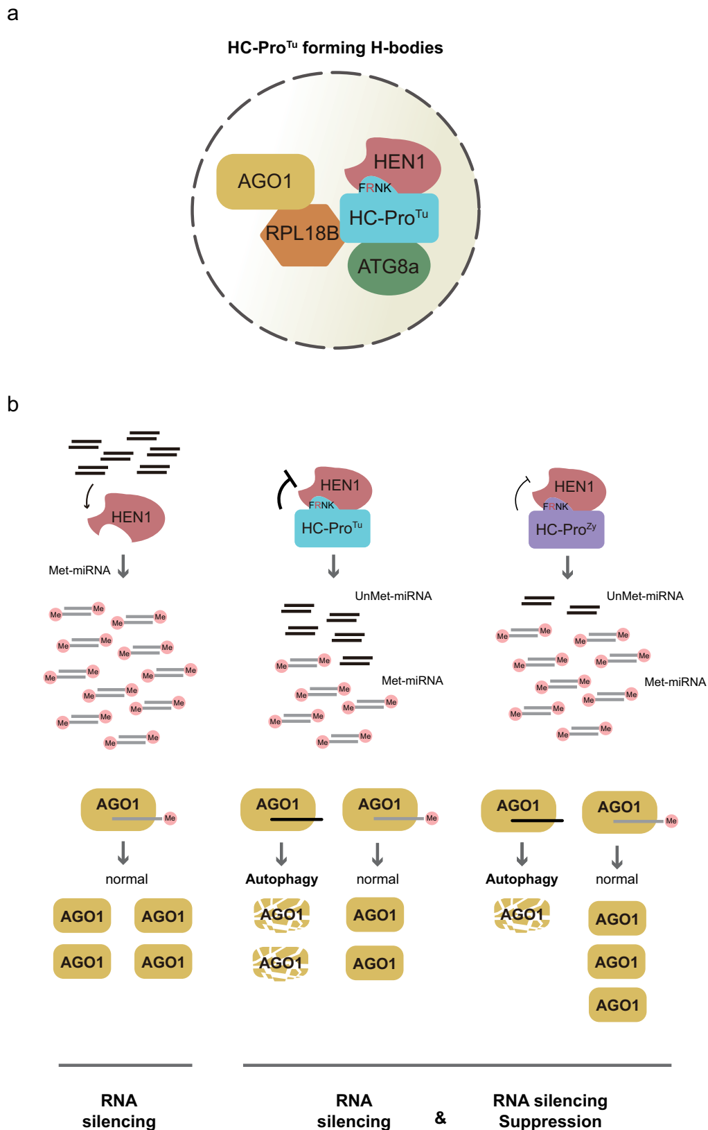
Fig. 7 | A working hypothesis model for the suppression of RNA silencing by HC-Pro Tu . a The inside of the H-body for HC-Pro interacts with RNA silencing components. b The working hypothesis for HC-Pro Tu -induced degradation of AGO1 suggests that HC-Pro Tu exhibits a heightened inhibitory effect on HEN1 methylation activity. This inhibition results in the incorporation of unmethylated miRNAs (unMet-miRNAs) into AGO1 complexes, which subsequently activate autophagy pathways, leading to the degradation of AGO1.
