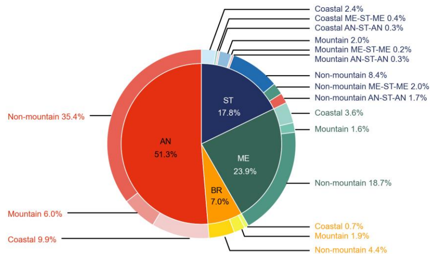
Fig. 1 | The proportion of global alluvial channel patterns. The length proportion of four channel types in different regions (i.e., non-mountain, mountain, and coastal) are shown using pie charts. AN: anabranching, BR: braided, ME: meandering, ST: straight. AN-ST-AN: the straight channel is connected to two or more anabranching channels, ME-ST-ME: the straight channel is connected to two or more meandering channels. Coastal reaches are defined as regions within 25 km of the coastline 33 or within deltas 34 , with elevation less than 100 m. Mountainous reaches are regions intersected by both the 1 km buffer boundaries of the mountain 35,36 and the unconsolidated sediments map 37 . The remaining reaches are classified as non-mountainous reaches which are not intersected by the 1 km buffer boundaries of the mountain map.
