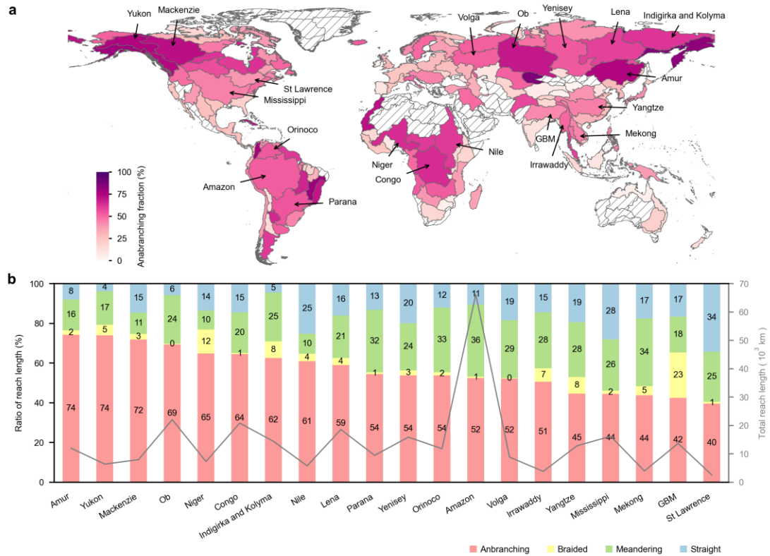
Fig. 3 | Basin-level statistics for non-mountainous alluvial channels. a , Fraction of anabranching channels at the basin scale in non-mountainous regions. The locations of the 20 largest river basins with rivers exceeding a mean annual discharge of 1000 \text{ m}^3 \text{ s}^{-1} are indicated on the global map. Hatch areas denote basins with no anabranching channels detected in non-mountains. b , The proportion of four channel types for the 20 largest river basins, sorted in descending order of anabranching fraction. The proportions for each channel type within their non-mountainous basin areas are annotated on their respective bars. The grey line signifies the total reach length within each non-mountainous basin. GBM, Ganges-Brahmaputra-Meghna River. The level-3 basin boundaries were provided by HydroBASIN dataset 103 . Basemaps in a from Natural Earth (naturalearthdata.com). Map created using Python 3.9.
