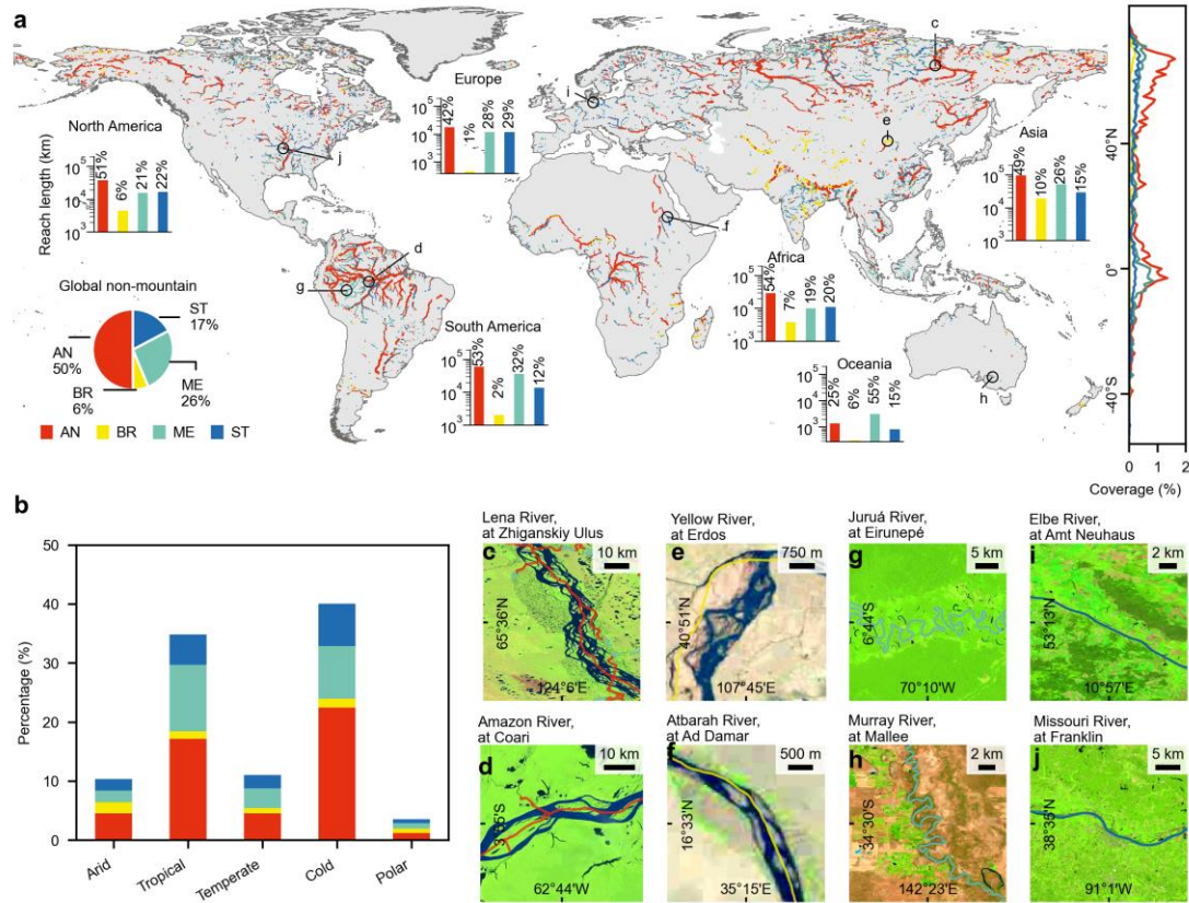
Fig. 2 | The distribution of global non-mountainous alluvial channel patterns. Non-mountainous alluvial channel patterns are mapped on a . Latitudinal profiles summarizing (by 1°) the proportion of different channel types (i.e., AN: anabranching, BR: braided, ME: meandering, ST: straight) as a percentage of the total non-mountainous reach length are shown on a . The proportions of different channel types using pie charts and bar plots are presented within panel a . Physio-climatic distribution on four types as a percentage of non-mountainous reach length is visualized on b . Planform characters of the channels are displayed in c-j (anabranching: c , d ; braided: e , f ; meandering: g , h ; straight: i , j ) using Landsat true-color images. Basemaps in a from Natural Earth (naturalearthdata.com). Map created using Python 3.9.
