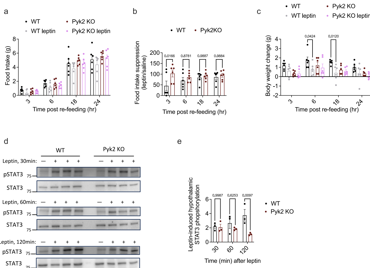
Fig. 6 | Pyk2 KO mice have impaired leptin sensitivity. a–c Fasted lean wild-type and Pyk2 KO mice were treated (ip) with vehicle or leptin, and food intake and body weights were followed for 24 h. a Time course of food intake, b food intake presented as normalized to the respective vehicle groups, and c weight change of the animals ( a–c , n = 6 mice per group). d , e Hypothalamic STAT3 phosphorylation was
