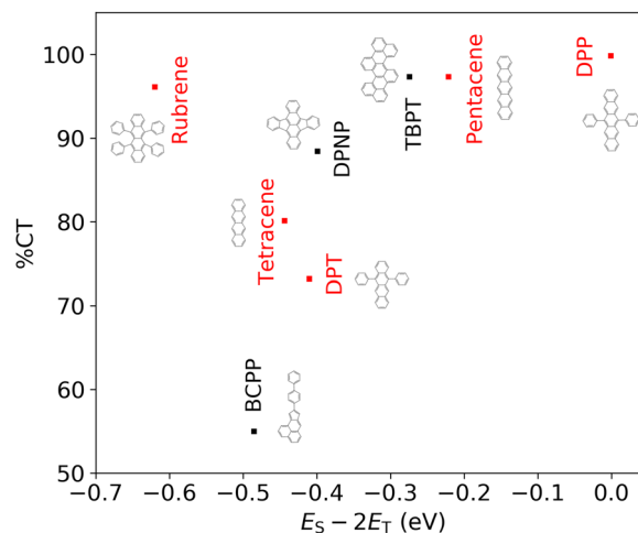
Fig. 7 2D descriptor of SF performance. BCPP, TBPT, and DPNP compared to known SF materials, colored in red, with respect to a two-dimensional descriptor calculated with GW + BSE. The thermodynamic driving force for SF ( E_S - 2E_T ) is displayed on the x-axis and the singlet exciton charge transfer character (%CT) is displayed on the y-axis.
