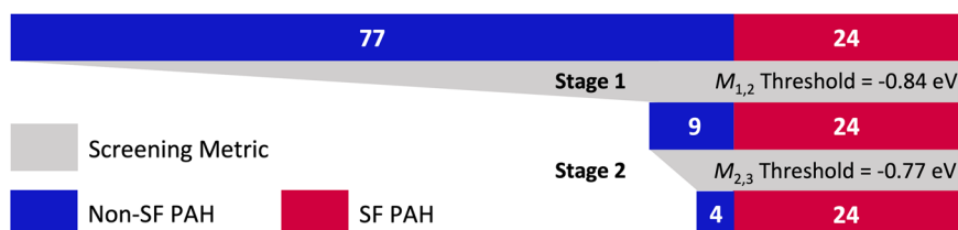
Fig. 4 Hierarchical screening workflow. Schematic of the hierarchical screening workflow based on models M_{1,2} and M_{2,3} , applied to the PAH101 set.
