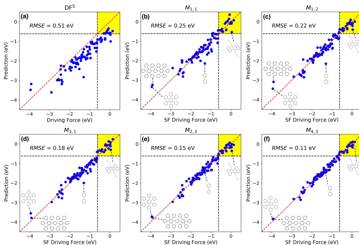
Fig. 3 Correlation plots of selected models. Model prediction as a function of the GW+BSE SF driving force for a the baseline model, DF^S , and the five models on or close to the Pareto front: b M_{1,1} , c M_{1,2} , d M_{3,1} , e M_{2,3} , and f M_{4,3} . The training set RMSE and molecular structures of four outliers are also shown. The true positive region for SF candidates is colored in yellow.
