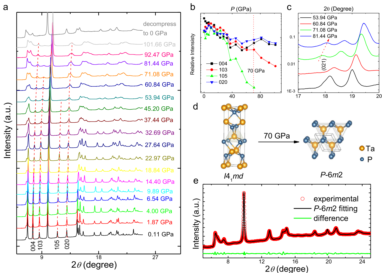
Fig. 4 HP-XRD results and the high-pressure structure of TaP. a The high-pressure x-ray diffraction of TaP up to 101.66 GPa. The red dashed lines highlight the evolution of some selected peaks. b Relative diffraction intensity of four selected peaks normalized by that of the (112) peak vs. applied pressures. c The emergence of (021) peak belonging to the P-6m2 structure when the pressure exceeds 71.08 GPa (green line), which clearly indicates the structure phase transition. d Crystal structures of I4_1md and P-6m2 phases (elaborated using the VESTA software 39 ). TaP adopts I4_1md space group at ambient pressure and transforms to P-6m2 at about 70 GPa. This high-pressure phase can be reserved after external pressure released. e XRD data after decompressing (symbols) and the fitting result using the P-6m2 structure (black solid line)
