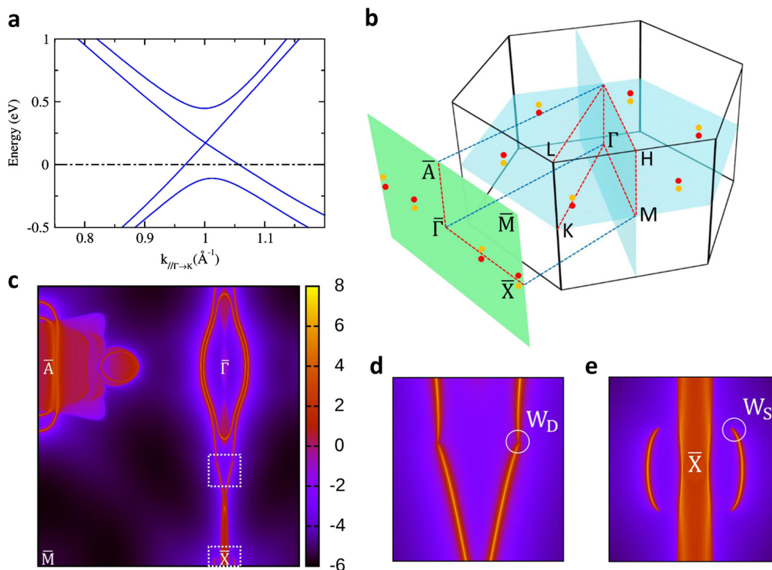
Fig. 5 Electronic structures and surface states of the TaP P\text{-}6m2 phase at 70 GPa. a The band structures around the Weyl point along the path parallel with \Gamma\text{-K} high-symmetry line. b The bulk Brillouin zone and its projection on (100) direction. The Weyl points with opposite chirality are marked by red and yellow, respectively. c–e The Fermi surface of TaP (100)-surface states of P atom termination. And the chemical potential is set at energy of Weyl point. W_S and W_D mark the projection points of single Weyl point and two Weyl points of same chirality, respectively
