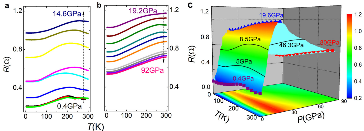
Fig. 1 Temperature-dependent resistance under pressures. a Temperature dependence of resistance for pressures from 0.4 to 14.6 GPa, and those from 19.2 to 92.0 GPa are shown in b . The inset of b shows the magneto-resistance at 4.5 K up to 8 T under different pressures. c The three-dimensional contour plot of resistance vs. temperature under different pressures
