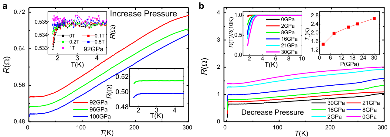
Fig. 3 Temperature-dependent resistance with increasing and decreasing pressures. a Temperature-dependent resistance from 92 to 100 GPa with increasing pressure. The R(T) curves under different pressures with decreasing pressure are shown in b . The upper-left inset in a shows the resistance vs. temperature under different fields at 92 GPa, and the lower-right inset shows the enlarged view of the data measured near 71 GPa in low-temperature region. The superconductivity is further evident by a sharp 75% drop of the normal state resistance under 30 GPa, as shown in the left inset in b . The inset on the right-hand side in b shows the pressure dependence of T_c in decreasing pressure
