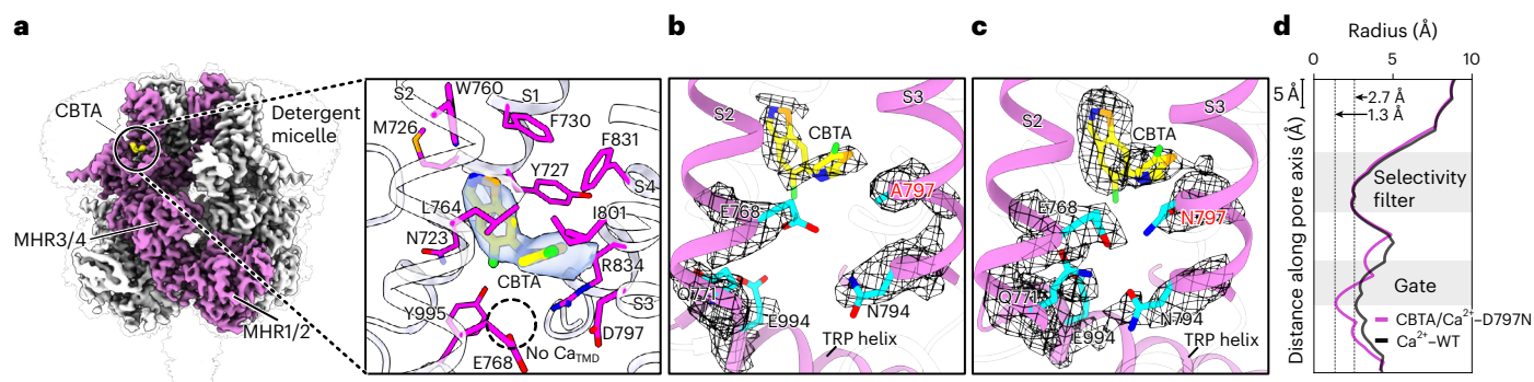
Fig. 3 | CBTA binds to TRPM5 independently of \text{Ca}_{\text{TMD}} . a , The structure of CBTA/EGTA-TRPM5. Left: cryo-EM map of TRPM5 with one subunit colored in magenta. Right: a close-up view of the S1–S4 domain. The CBTA molecule is shown using stick representation and colored in yellow. The cryo-EM density for CBTA is shown using a semitransparent surface. b , A close-up view of the \text{Ca}_{\text{TMD}}
