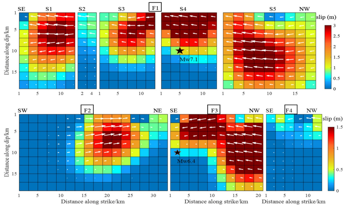
Figure 10. The slip distribution of the Mw 6.4 foreshock and the Mw 7.1 main shock from inversion of T71-D coseismic displacements.
