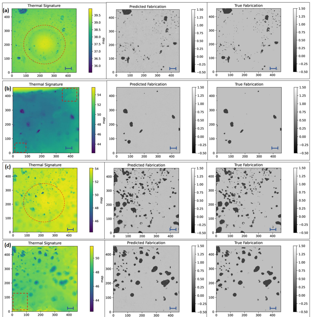
Figure 2. Thermal image, corresponding predicted, and true image for (a) 2.5% G Planetary, (b) 2.5% G Hand, (c) 10% G Planetary, (d) 10% G Hand. Thermal image is manually fed in image processing to remove artifacts or voids or blurriness (scale bar = 1000 microns, enclosing red circle area remarks artifact due to container mark, enclosing rectangle area remarks void area). The thermal image is then fed into machine learning model to obtain the true fabrication. By feeding a few thermal signatures, this learning method can show true fabrication in a really quick manner.
