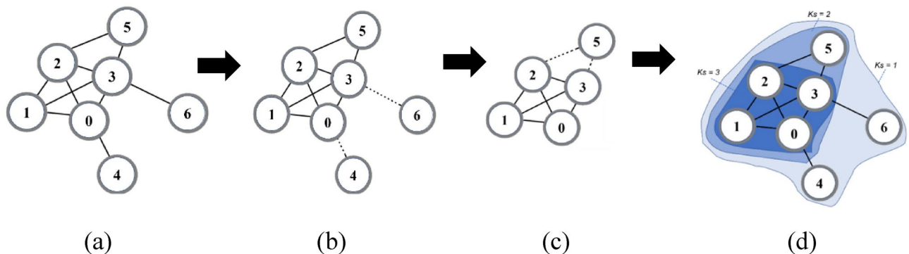
Figure 1. (a) A network with 7 nodes and 10 edges. (b) Removing of the most outer layer, which is node 4 and 6. (c) Removing of the next outer layer, which is node 5. (d) Summary of the Ks -territory of all the nodes in the network.
