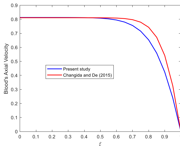
Figure 12. Model validation.
