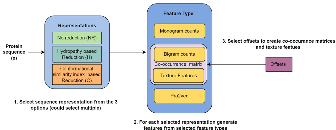
Figure 2. Feature extraction framework.
