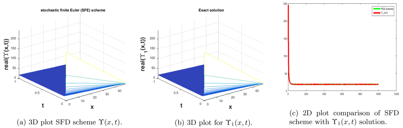
Figure 5. The subfigure (a) shows the 3D behavior of SFD scheme, subfigure (b) shows the stochastic exact solitary wave solution while subfigure (c) shows the 2D comparison of SFD scheme with exact solitary wave solution.
