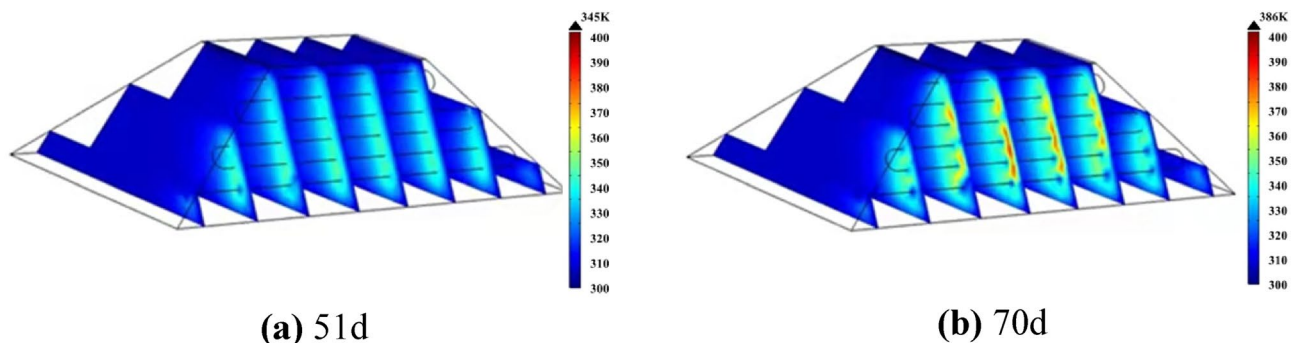
Figure 17. The temperature distribution of coal pile of arrangement of multi-row water-cooling steel pipes.
