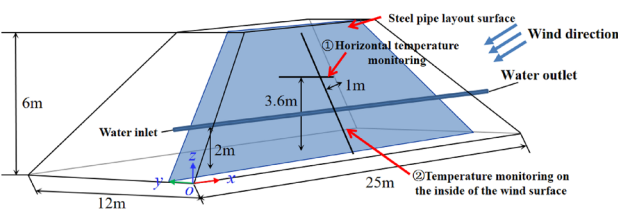
Figure 4. Coal pile geometry.
