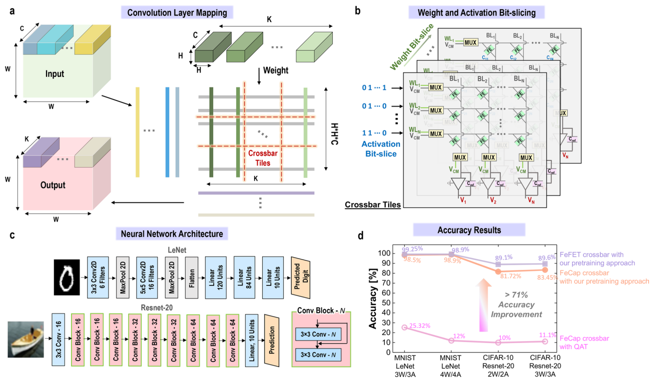
Figure 8. Pretraining approach for FeCaps-based neural network. (a) Convolution layer mapping to FeCap crossbars using Im2Col transform. (b) Demonstration of bit-slicing on input activations and stored weights for FeCap-based crossbars. (c) Neural network architectural layout of LeNet and Resnet-20 models. (d) Simulation results on MNIST and CIFAR-10 datasets for LeNet and Resnet-20 models comprised of FeCap and FeFET crossbars. FeCap crossbars based on Quantization-Aware Training (QAT) indicate lower accuracy. Accuracy evaluation of FeCap crossbars using our pretraining approach demonstrates significant accuracy improvement in FeCap-based neural network, comparable to the FeFET baseline. Note that QAT represents the training approach that only trains for quantization without considering the leakage of FeCaps.
