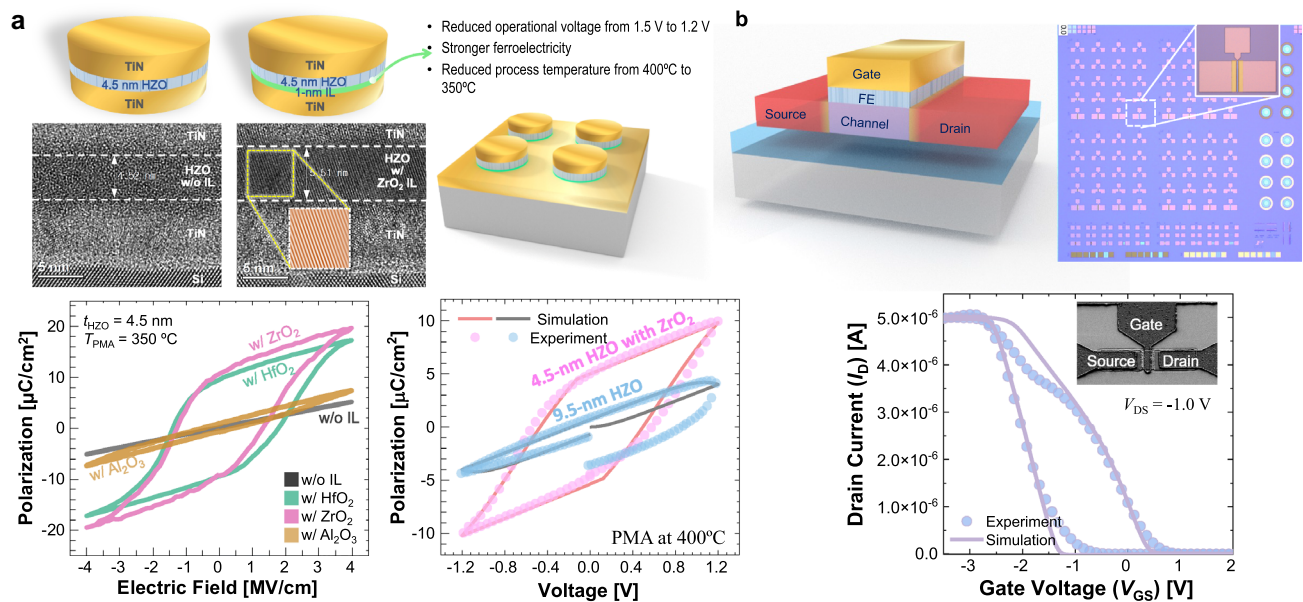
Figure 2. Schematics and performances of our fabricated FeCaps and FeFET. (a) High-resolution transmission electron microscopy (HR-TEM) images of FeCaps having a 4.5-nm HZO layer without an IL (left) and with 1-nm \text{ZrO}_2 IL (right). Polarization-electric field plots of the FeCaps having different IL materials along with 4.5-nm HZO (annealing temperature was 350^\circ\text{C} ). Without IL, the HZO layer remained as paraelectric material under the given annealing temperature. Simulation model fitting results with 9.5-nm and 4.5-nm HZO thicknesses devices. (b) Optical microscope image of our fabricated die. Fitted FeFET transfer curve obtained from the simulation model compared with the experimental data (inset: Scanning Electron Microscope (SEM) image).
